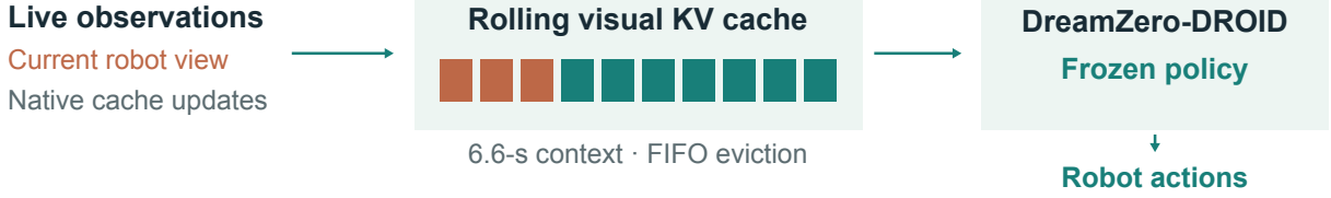
Figure 9 | Training-free Embed2ICL. Robota-Embed retrieves candidate VLA clips, and the Reranking Agent selects a task-relevant reference containing completion evidence. Its video initializes DreamZero-DROID’s visual key-value cache. The policy remains frozen while live observations update the cache during execution.
