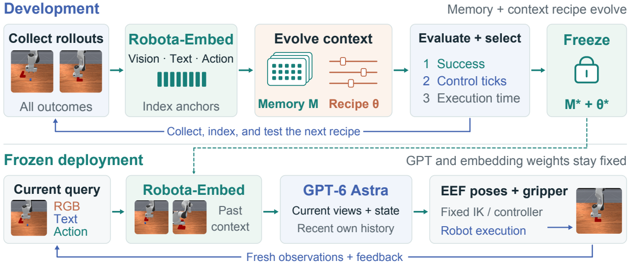
Figure 7 | Embed2Evolve. Development grows memory and optimizes its use; testing fixes both. GPT-6 Astra proposes actions for a fixed controller. The model comparison replaces Robota-Embed in both phases. Images show the PullCubeTool task.
