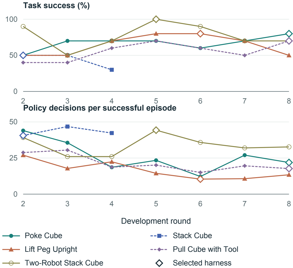
Figure 15 | Task-wise development trajectories. Success uses ten trials per round; decisions average that round's successful trials. Hollow diamonds mark selected harnesses. Lines connect evaluated candidates, not necessarily parent-child configurations.
