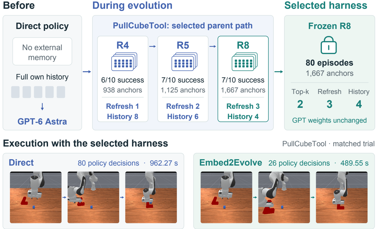
Figure 14 | From Direct control to a selected harness. PullCubeTool’s R4 → R5 → R8 parent–child sequence grows memory while reducing retained history and retrieval frequency. The bottom filmstrips show the same fresh-test initialization completed successfully by both systems. Task execution time includes API waits.
