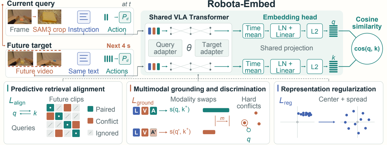
Figure 2 | Robota-Embed architecture and objectives. Each query is paired with the next four seconds of recorded video and actions. Three objective groups train a joint VLA space.
