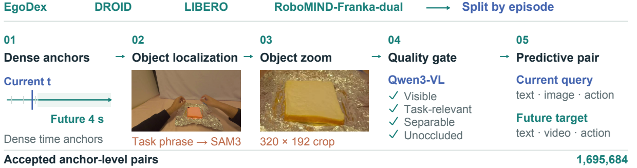
Figure 3 | Multi-source training-data curation. We split episodes before sampling anchors, localize and verify interaction crops, and pair accepted anchors with video and actions from the next four seconds. Query filtering uses only the instruction and current observations.
