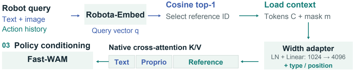
Figure 12 | Training-based Embed2ICL. Offline encoding caches each candidate’s retrieval vector, Context Tokens, and context mask. Online cosine top-1 search selects a reference and loads its tokens and mask. The prefilling adapter projects the tokens to Fast-WAM’s context width and appends them to the native text and proprioceptive conditioning for cross-attention.
