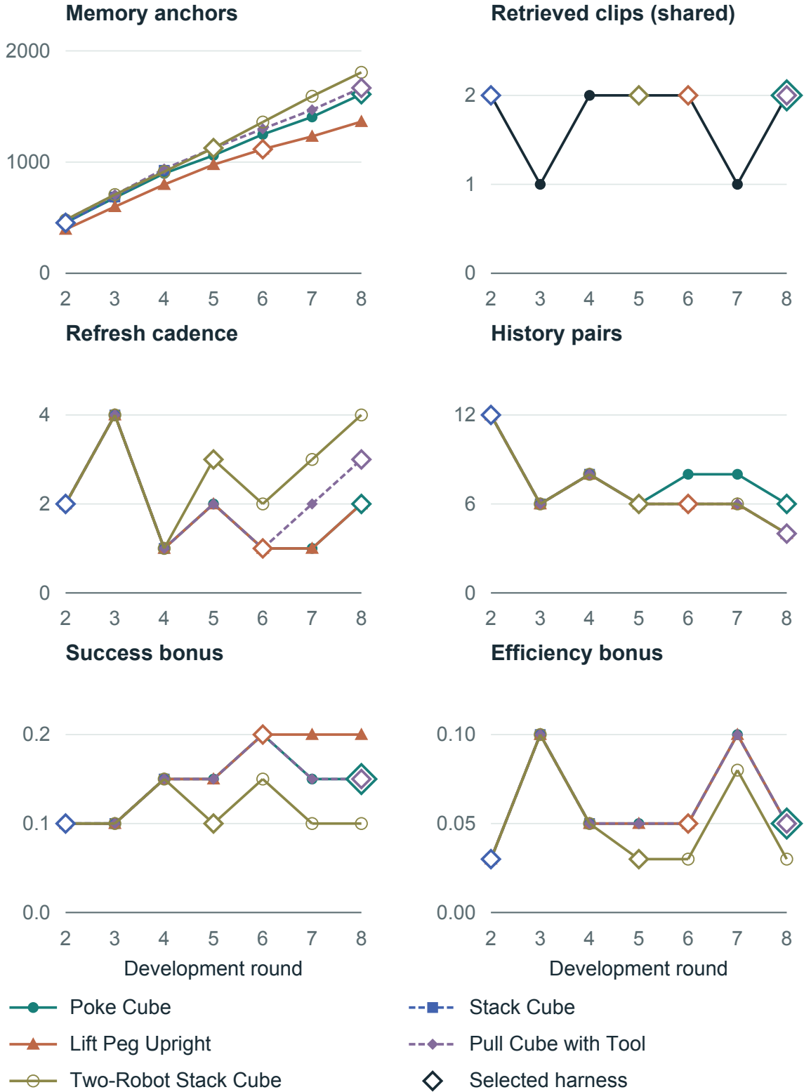
Figure 16 | Two evolving components: memory and context recipe. Per-task trajectories show memory size, retrieval count, refresh cadence, history, and ranking bonuses with fixed model weights. Hollow diamonds mark selected rounds; nested diamonds show coincident selections.
