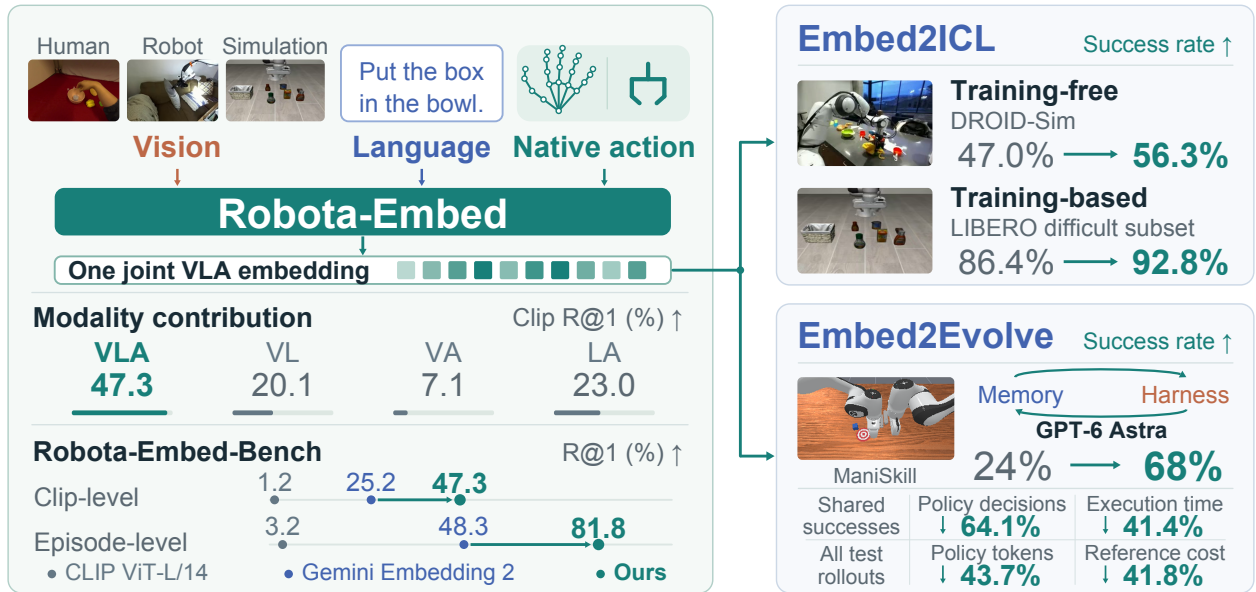
Figure 1 | One joint VLA embedding, two context applications. Robota-Embed jointly encodes vision, language, and native action from human, robot, and simulated experience to retrieve recorded continuations. Action improves retrieval beyond vision and language alone. Embed2ICL uses retrieved demonstrations to condition robot policies. Embed2Evolve grows task-local memory and refines how a fixed GPT-6 Astra policy uses it, improving success and efficiency relative to Direct.
