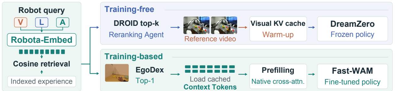
Figure 5 | Embed2ICL: one retriever, two policy interfaces. Reranked DROID videos warm up DreamZero’s visual cache; top-1 EgoDex matches supply Context Tokens for Fast-WAM’s native cross-attention. Retrieval vectors select experience; videos or tokens condition the policy.
