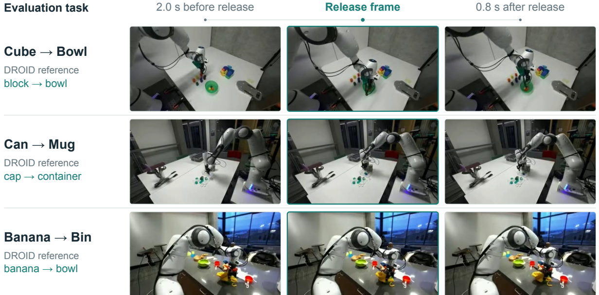
Figure 10 | DROID references for training-free Embed2ICL. Each row shows one task’s fixed reference from a single camera, before, at, and after the detected final gripper release. DreamZero-DROID receives all three synchronized four-second video streams.
