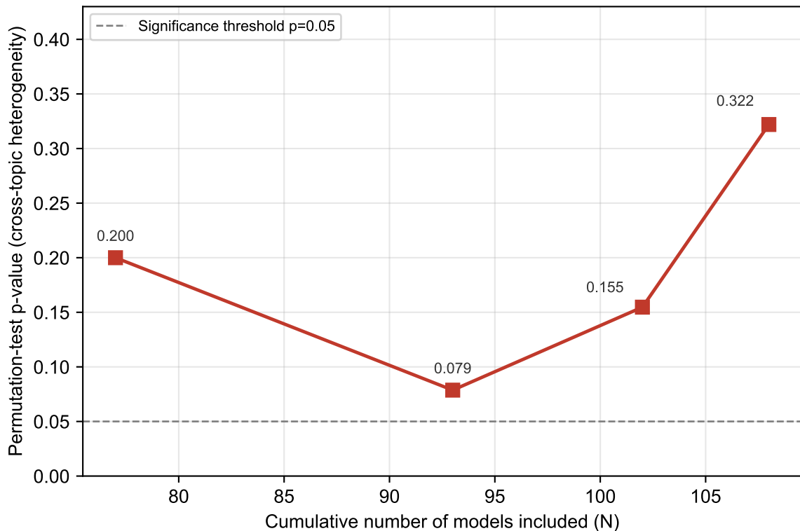
Figure 3. Non-monotonic trajectory of the cross-topic heterogeneity permutation-test p-value across 4 checkpoints
