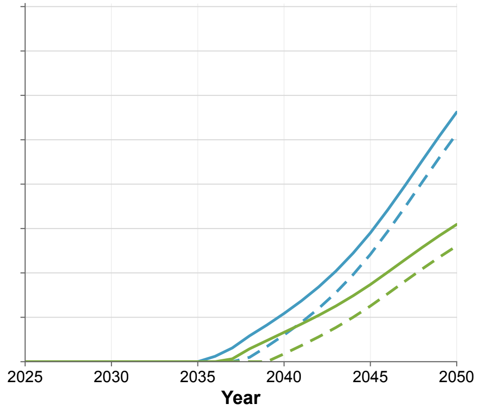
Policy Rollback
