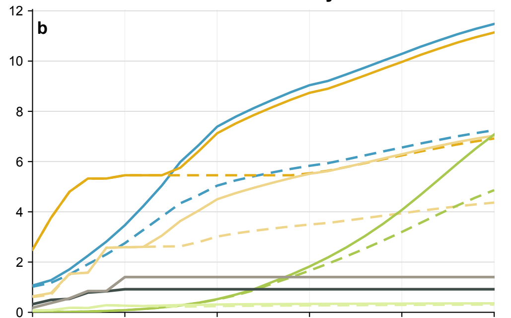
Rollback Policy
