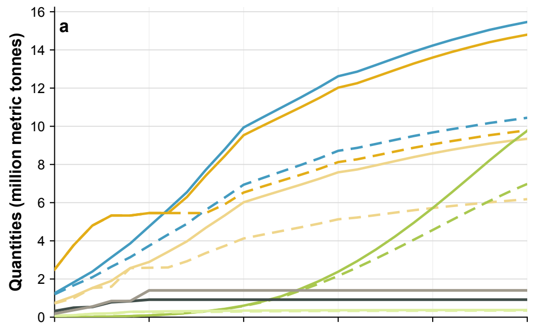
Baseline Policy
