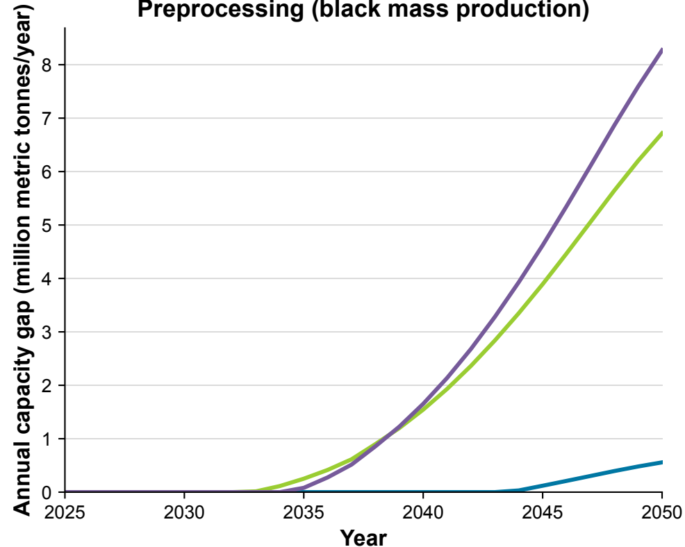
Preprocessing (black mass production)
