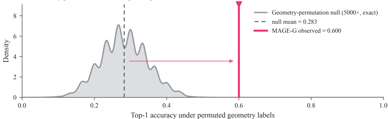
C. Geometry-permutation null (empirical p \approx 0.0002 )
