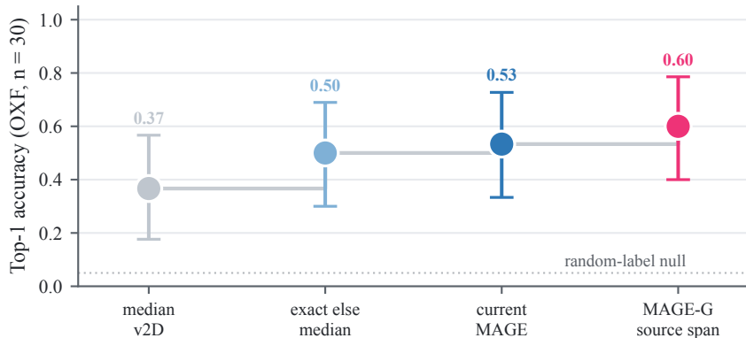
A. OXF geometry ladder (cumulative \Delta = +0.233 , CI [+0.034, +0.444] )
