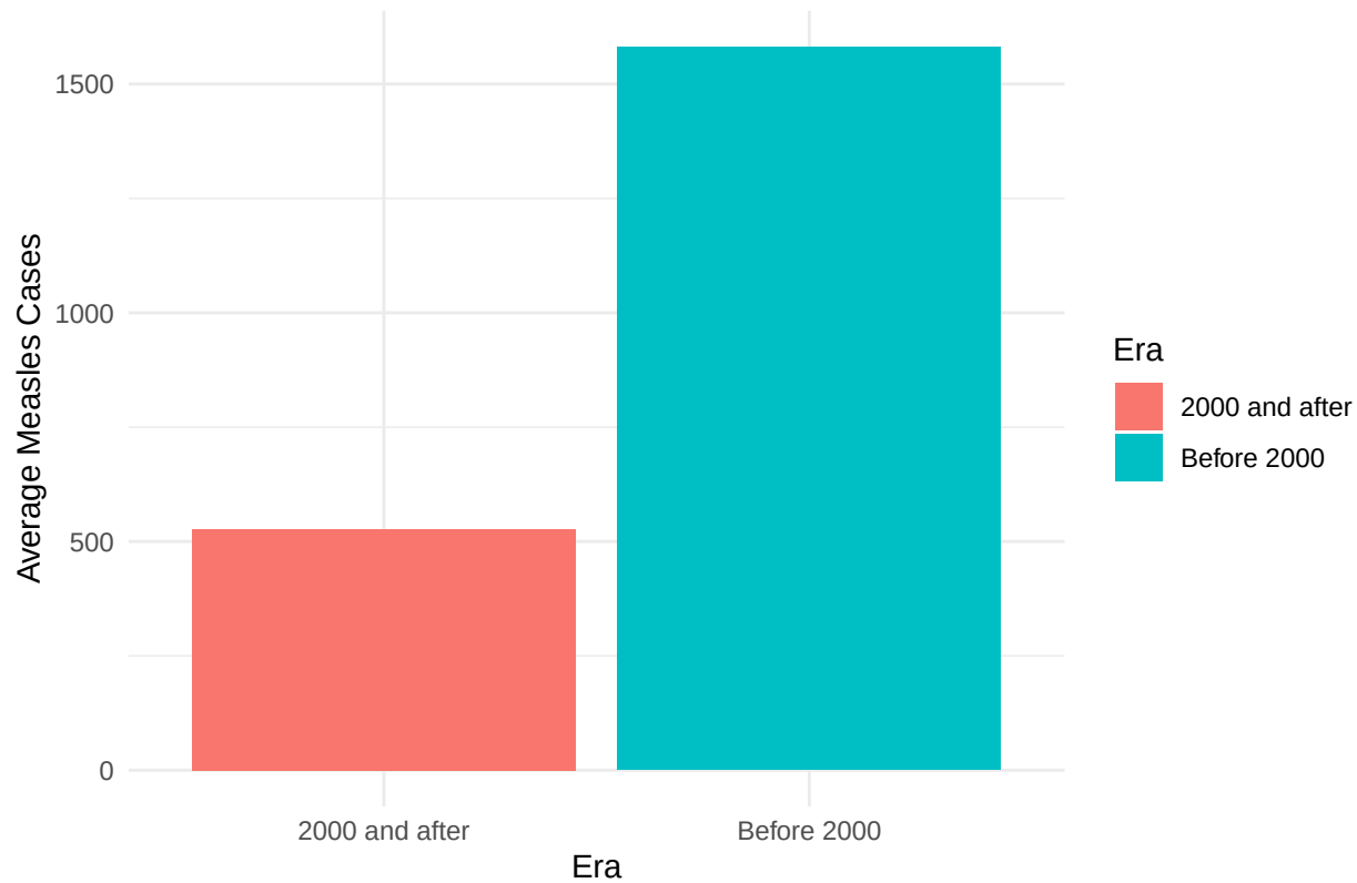
Average Measles Cases: Before vs After 2000
