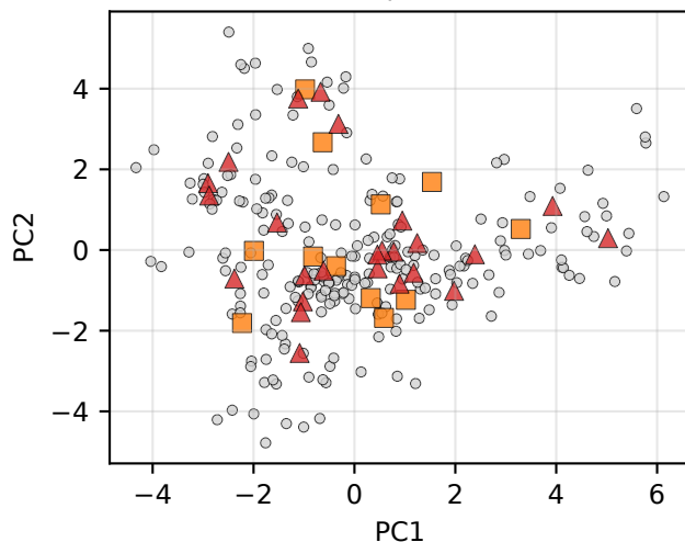
(b) Blind PCA found 0/12 | false-pos 12
