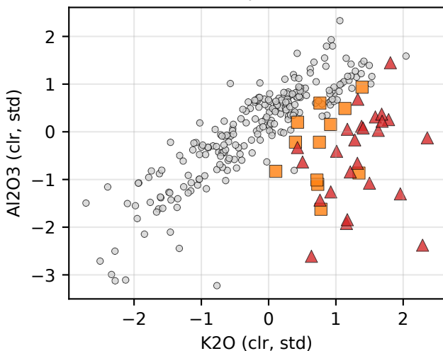
(c) Anchored TPP (15 anchors) found 7/12 | false-pos 5
