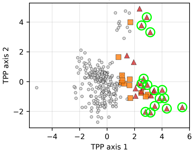
(c) Anchored TPP (15 anchors) found 7/12 | false-pos 5
