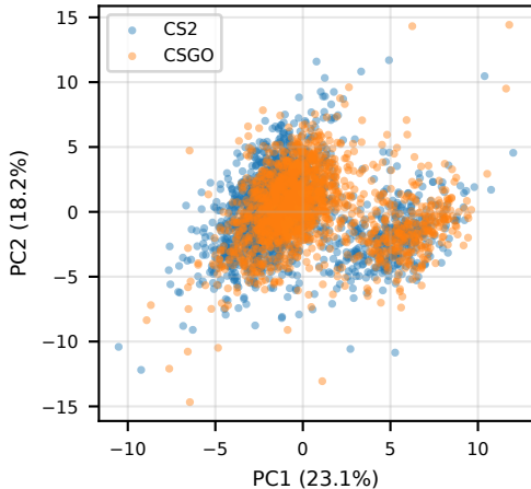
PCA by game version
