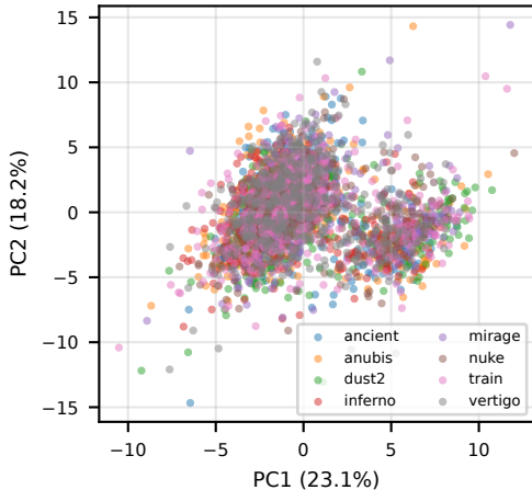
PCA by map
