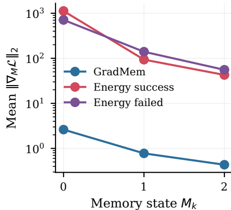
WRITE gradient scale
