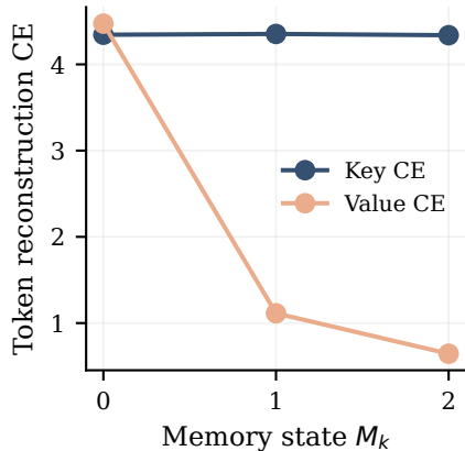
GradMem: forward WRITE
