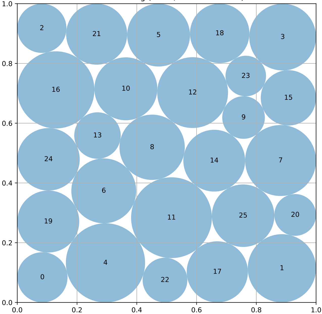
Circle Packing (n=26, sum=2.628824)
