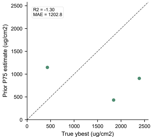
Ybest estimate
