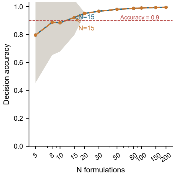
Decision learning curve
