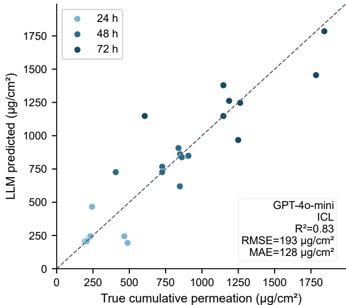
Best ICL parity plot
