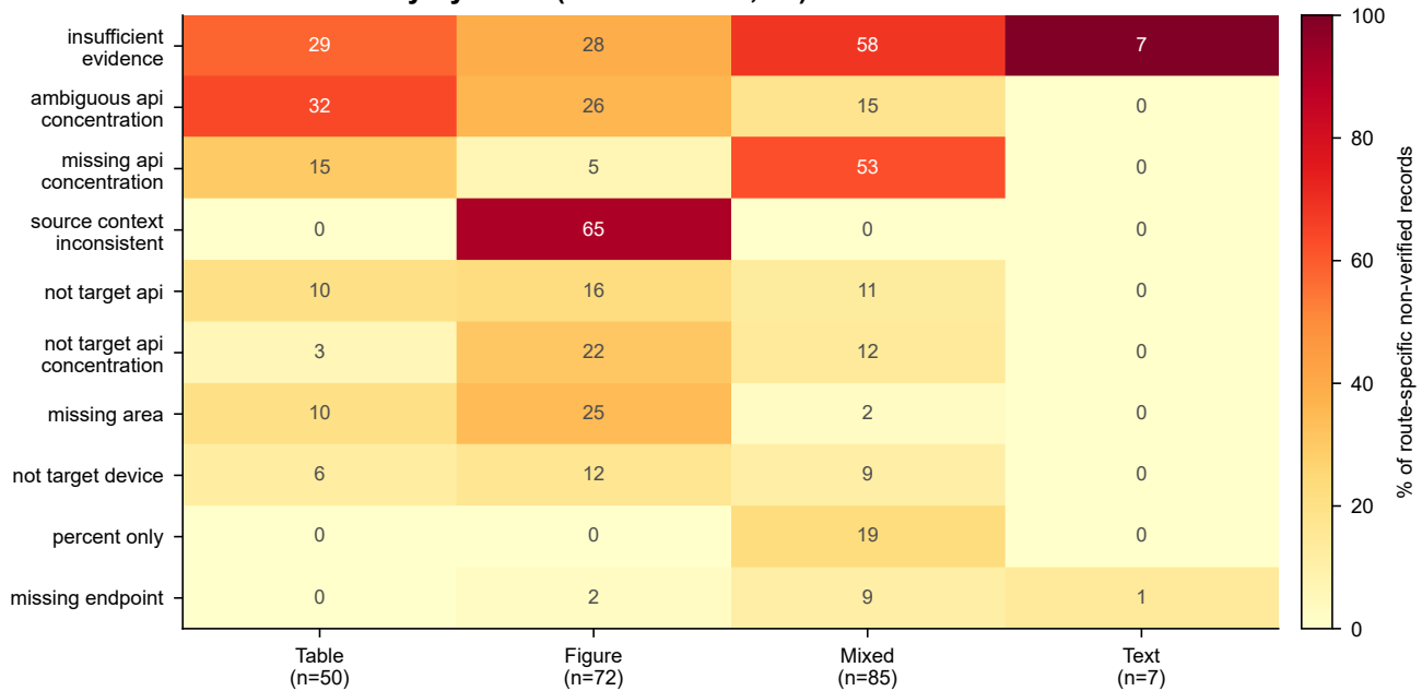
Failure taxonomy by route (GPT baseline, v2)
