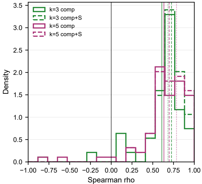
B. Few-shot Spearman distributions
