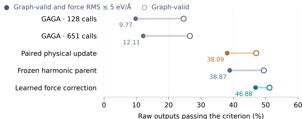
Figure 10: Graph support and physical quality on the same compositions. Open circles count graph-valid outputs; filled circles also require GFN2 force RMS at most 5 eV/Å. The gap shows graph-valid outputs above that force threshold. Every denominator includes all 512 attempts. The models have the distinct training histories and inference costs described in the text.
