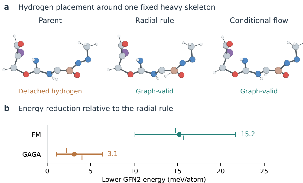
Figure 9: A conditional hydrogen flow learns more than attachment distance. Top: the same saved FM output before readout, after the radial rule, and after the learned flow. All atoms are shown with a shared camera and scale. Sticks are distance contacts in every panel, not inferred chemical bond orders. The example is selected by a fixed metadata hash among repaired, jointly graph-valid examples with at most 28 atoms; energy is not a selection criterion. Bottom: all-output energy reductions relative to the radial rule, with 95% composition-bootstrap intervals and the two fit-specific means. Carbon, hydrogen, nitrogen, oxygen, boron, and iodine are gray, white, blue, red, tan, and purple.
