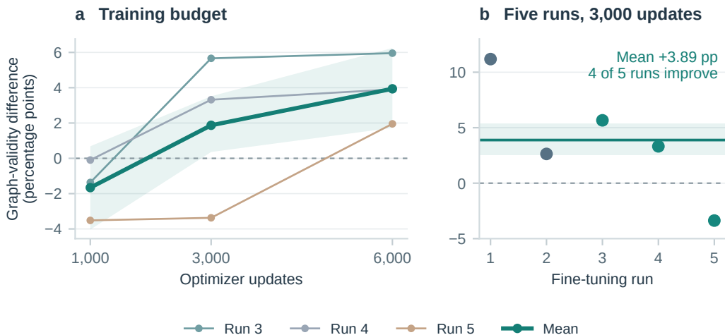
Figure 6: Source effects across training budgets and fine-tuning runs. Thin lines show all three new runs; the thick line is their mean. The right panel includes all five runs at 3,000 updates. Shading and the horizontal bar show 95% composition-bootstrap intervals conditional on the fitted models.
