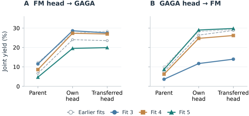
Figure 4: Direct transfer of correction weights. Each line follows one training pair through the uncorrected parent, its own fitted head, and the other model’s head. Dashed open markers show the two earlier pairs; colored filled markers show the three new pairs. Each setting contains 1,024 attempts per pair on the same 64 compositions. The source distribution and target backbone are preserved; the hydrogen readout is disabled.
