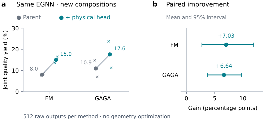
Figure 7: Physical correction transfers to independently trained EGNN generators. (a) Joint yield requires an inferred valid graph and GFN2 force RMS at most 5 eV/Å. Large circles show pooled rates; small crosses show the two fits. (b) Within-parent improvements with paired composition-bootstrap 95% intervals. Both algorithms receive the same TRAIN compositions, force-query budget, head architecture, and fitting schedule. All generated coordinates are unoptimized.
