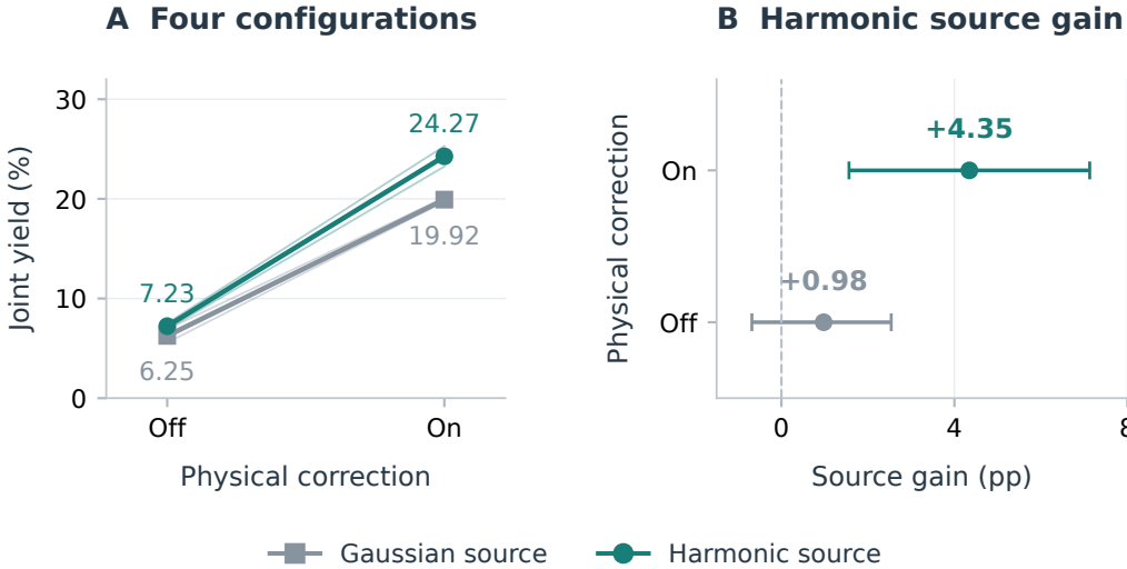
Figure 3: Contributions of the source and physical correction. (A) Mean joint yield for the four configurations; faint lines retain both training fits. (B) Harmonic-minus-Gaussian joint-yield gains, with nominal 95% intervals from resampling fits and compositions. Each configuration uses 2,048 outputs on the same 64 compositions and one network evaluation per velocity prediction.
