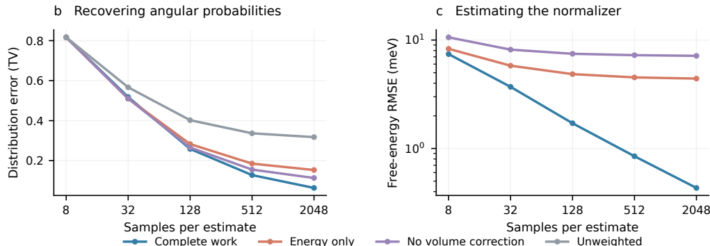
Figure 11: Work correction on controlled molecular rotors at 300 K. (a) Reference structures and the prescribed methyl rotations. (b,c) Angular-distribution and normalizer errors averaged over three molecules and two nonidentity maps, with 128 repetitions per case. Complete weights account for the proposal bias left by energy-only and incomplete weights. Unweighted samples have no free-energy estimator. Each target retains its angular reference restraint.
