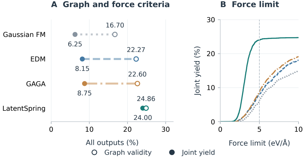
Figure 2: Generation quality on 64 unseen compositions. (A) Open markers show graph validity; filled markers show joint yield at the 5 eV/Å force threshold. The connecting segment counts graph-valid outputs above that threshold. (B) Empirical joint-yield curves computed from every saved force score; the dashed line marks 5 eV/Å. Colors and line styles identify the same methods in both panels. Gaussian FM and EDM use two fits (2,048 outputs per method); GAGA and LatentSpring use five (5,120). The hydrogen readout is disabled.
