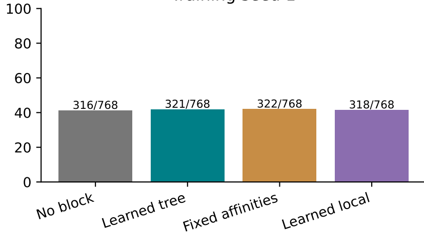
Training seed 1
