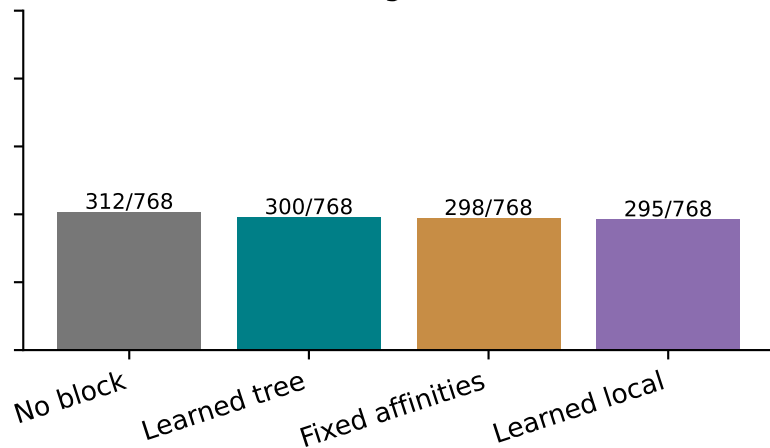
Training seed 2
