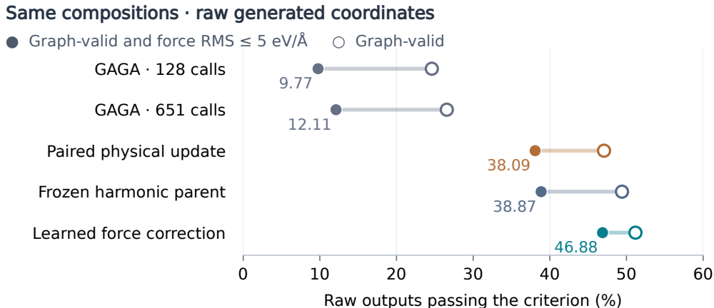
Figure 11: Graph validity and joint yield on the common panel. Open circles show graph validity; filled circles also require GFN2 force RMS at most 5 eV/Å. Connecting segments show the gap between the two criteria. Rates use all 512 attempts. Training histories and inference costs differ across systems, as described in the text.
