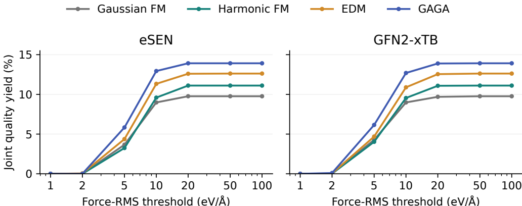
Figure 13: Joint yield versus force threshold, pooling two initializations and 64 compositions. All attempts contribute to the denominator. GAGA has the highest pooled yield at most nontrivial thresholds under both potentials.
