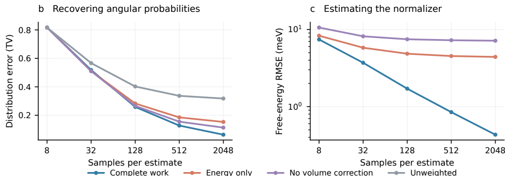
Figure 10: Work correction on controlled molecular rotors at 300 K. (a) Reference structures and the prescribed methyl rotations. (b,c) Angular-distribution and normalizer errors averaged over three molecules and two nonidentity maps, with 128 repetitions per case. Complete weights account for the proposal bias left by energy-only and incomplete weights. Unweighted samples have no free-energy estimator. Each target retains its angular reference restraint.
