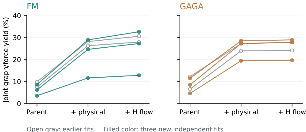
Figure 2: Completed physical-correction and hydrogen-readout comparisons in each of five training fits. Gray open markers identify the two earlier fits; filled markers identify the three new fits. Each line follows the same parent through correction and hydrogen readout. This figure reports the completed head experiments, separate from the combined-design diffusion comparison in Table 3.
