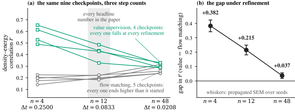
Figure A1: The paired resolution sweep. The same nine checkpoints — five flow-matching controls (seeds 1–5) and four value runs (seeds 1, 2, 3, 5) — re-scored at n = 4 , n = 12 and n = 48 ODE steps on identical parents, identical displacements and a pinned evaluation seed. (a) Per checkpoint: all four value checkpoints fall at every refinement, and all five flow-matching checkpoints end higher at n = 48 than at n = 4 , three of them monotonically. (b) The arm gap decays +0.382 \rightarrow +0.215 \rightarrow +0.037 . Each point is the difference of the two arm means over independently trained seeds, five control and four value, and each whisker is the propagated standard error over those seeds, a descriptive SEM rather than a confidence interval. Every number reported elsewhere in the paper is computed at n = 12 . The value loss was itself computed at n = 4 , so one reading of the decay is that the ordering the term teaches is expressed most strongly in the object the coarse estimator reports; that is offered as a reading and not as a demonstrated mechanism. What the analysis establishes is that the estimator is sensitive to solver resolution. It does not distinguish model-dependent numerical error from an effect learned under the four-step training estimator.
