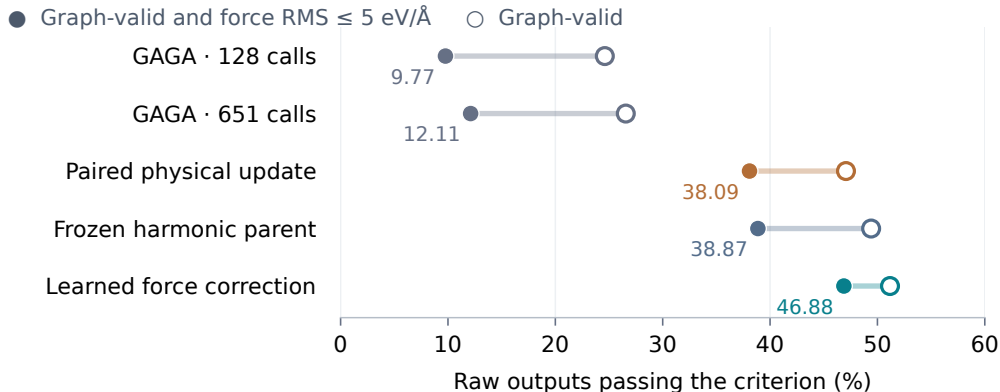
Figure 9: Graph support and physical quality on the same compositions. Open circles count graph-valid outputs; filled circles also require GFN2 force RMS at most 5 eV/Å. The gap shows graph-valid outputs above that force threshold. Every denominator includes all 512 attempts. The models have the distinct training histories and inference costs described in the text.
