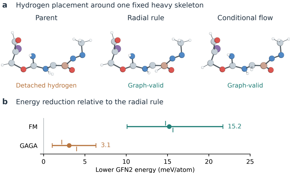
Figure 8: A conditional hydrogen flow learns more than attachment distance. Top: the same saved FM output before readout, after the radial rule, and after the learned flow. All atoms are shown with a shared camera and scale. Sticks are distance contacts in every panel, not inferred chemical bond orders. The example is selected by a fixed metadata hash among repaired, jointly graph-valid examples with at most 28 atoms; energy is not a selection criterion. Bottom: all-output energy reductions relative to the radial rule, with 95% composition-bootstrap intervals and the two fit-specific means. Carbon, hydrogen, nitrogen, oxygen, boron, and iodine are gray, white, blue, red, tan, and purple.
