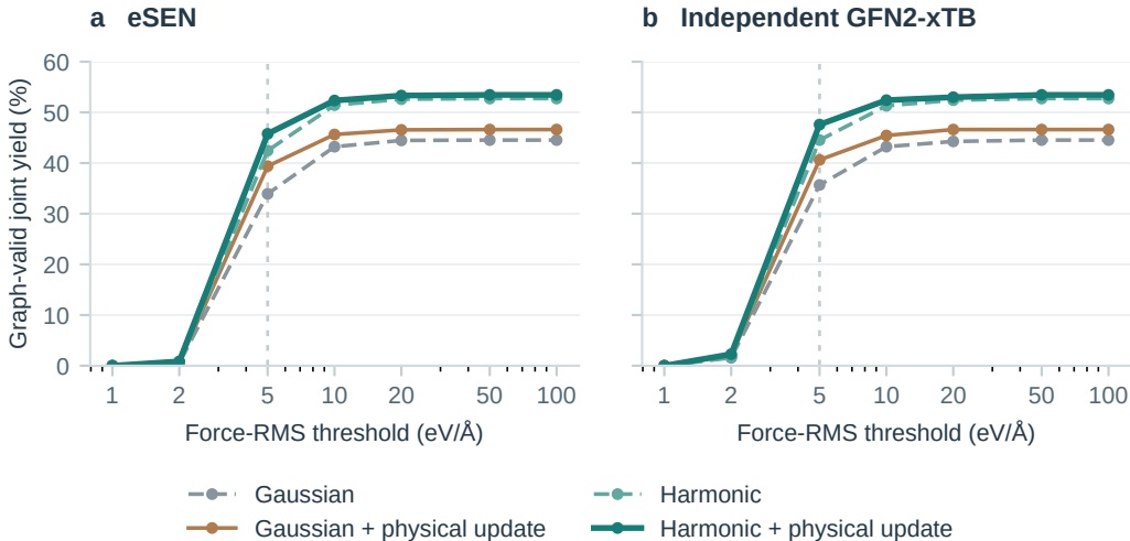
Figure 12: Joint graph-validity and residual-force yield for both sources, with and without the paired physical update. The denominator includes every raw generation attempt. Each threshold is applied to the RMS atomic-force magnitude in \text{eV}/\text{\AA} , and both potentials use the same threshold grid. No coordinates are optimized before evaluation.
