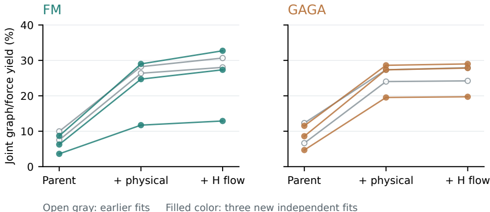
Figure 2: Every fitted model in the replication study. Each line follows one fixed parent through physical correction and the hydrogen readout. Gray open markers identify earlier fits; filled markers identify the three new fits. The models are compared on identical compositions and all attempts remain in the denominator.
