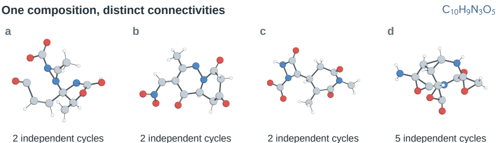
Figure 5: Different connectivities generated from the same atomic composition by the paired-update variant of LatentSpring. The initial trees have no cycles, but the generated molecules can contain rings. We show the first four graph-valid outputs with distinct connectivities for the first CHON composition with valid outputs in run 1 of the 24-composition set. Examples are not selected by energy or altered by geometry optimization. The number of independent cycles is the inferred edge count minus the atom count plus one.
