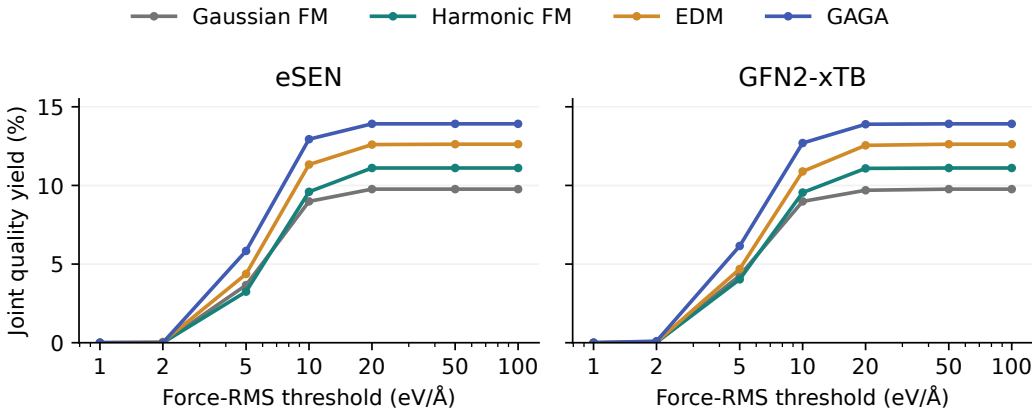
Figure 11: Fraction of all attempts that are graph-valid and have force RMS below the indicated threshold. Curves pool both independent initializations and all 64 compositions. GAGA has the highest pooled yield at most nontrivial thresholds under both potentials.
