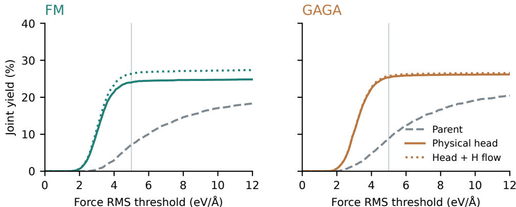
Figure 7: Joint yield as the force threshold varies, averaged over all five fits. The vertical reference marks the prespecified 5 eV/Å endpoint. These curves are descriptive; no threshold is selected from them.
