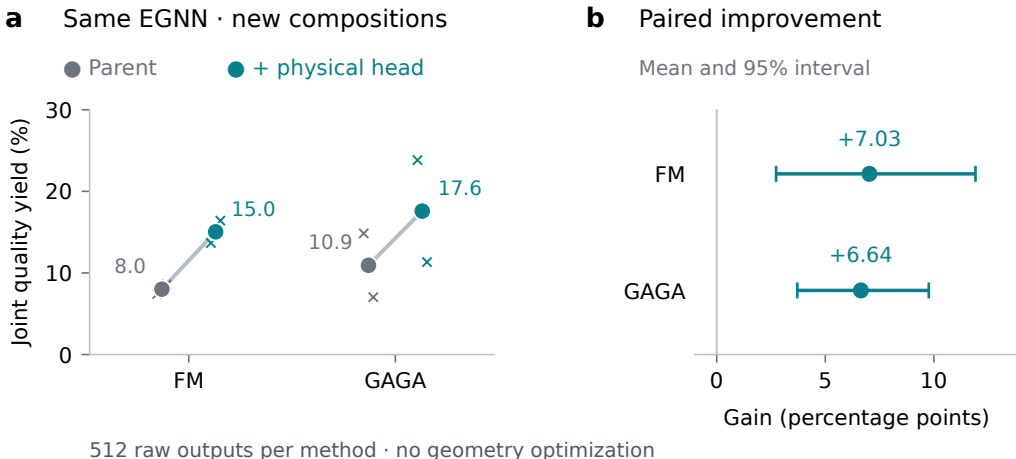
Figure 6: Physical correction transfers to independently trained EGNN generators. (a) Joint yield requires an inferred valid graph and GFN2 force RMS at most 5 eV/Å. Large circles show pooled rates; small crosses show the two fits. (b) Within-parent improvements with paired composition-bootstrap 95% intervals. Both algorithms receive the same TRAIN compositions, force-query budget, head architecture, and fitting schedule. All generated coordinates are unoptimized.
