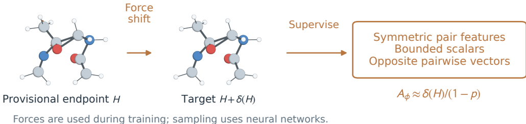
Figure 1: LatentSpring learns physical corrections to predicted endpoints. (a) A recorded harmonic source and corrected FM output for neutral singlet C10H5FN2O2 , shown with the same camera and scale. Dashed source edges are the actual sampled auxiliary tree; output bonds are inferred from coordinates. Composition, charge, and spin are the inputs; coordinates are the output. (b) A separate saved training endpoint and its force-shifted target. Sticks here are distance contacts. Arrows show recorded force directions with a common display scale; coordinate shifts are not exaggerated. The correction network learns from current coordinates, predicted endpoints, atom identities, and progress. Every backbone parameter remains fixed during this stage. Carbon, hydrogen, nitrogen, oxygen, and fluorine are gray, white, blue, red, and green.
