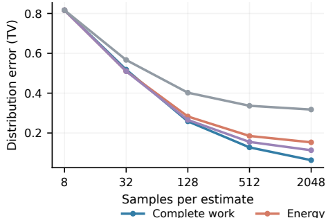
Figure 10: Work correction on controlled molecular rotors at 300 K. (a) Reference structures and the prescribed methyl rotations. (b,c) Angular-distribution and normalizer errors averaged over three molecules and two nonidentity maps, with 128 repetitions per case. Complete weights account for the proposal bias left by energy-only and incomplete weights. Unweighted samples have no free-energy estimator. Each target retains its angular reference restraint.
