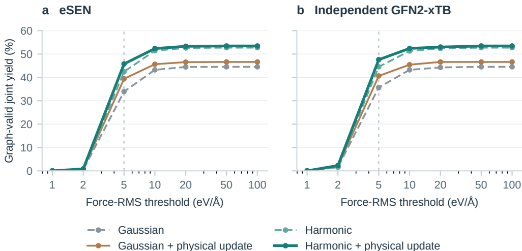
Figure 8: Joint graph-validity and residual-force yield for both sources, with and without the paired physical update. The denominator includes every raw generation attempt. Each threshold is applied to the RMS atomic-force magnitude in \text{eV}/\text{\AA} , and both potentials use the same threshold grid. No coordinates are optimized before evaluation.
