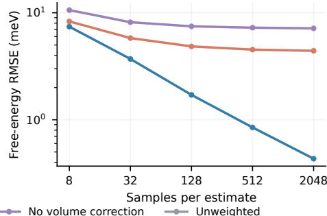
Figure 6: Work correction on controlled molecular rotors at 300 K. (a) Reference structures and the prescribed methyl rotations. (b,c) Angular-distribution and normalizer errors averaged over three molecules and two nonidentity maps, with 128 repetitions per case. Complete weights account for the proposal bias left by energy-only and incomplete weights. Unweighted samples have no free-energy estimator. Each target retains its angular reference restraint.
