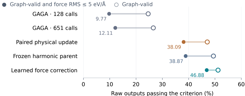
Figure 5: Graph support and physical quality on the same compositions. Open circles count graph-valid outputs; filled circles also require GFN2 force RMS at most 5 eV/Å. The gap shows graph-valid outputs above that force threshold. Every denominator includes all 512 attempts. The models have the distinct training histories and inference costs described in the text.
