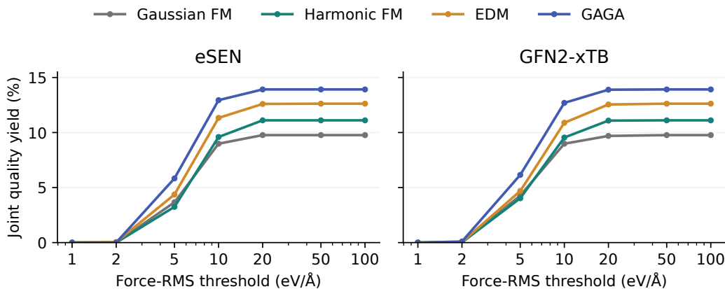
Figure 7: Fraction of all attempts that are graph-valid and have force RMS below the indicated threshold. Curves pool both independent initializations and all 64 compositions. GAGA has the highest pooled yield at most nontrivial thresholds under both potentials.
