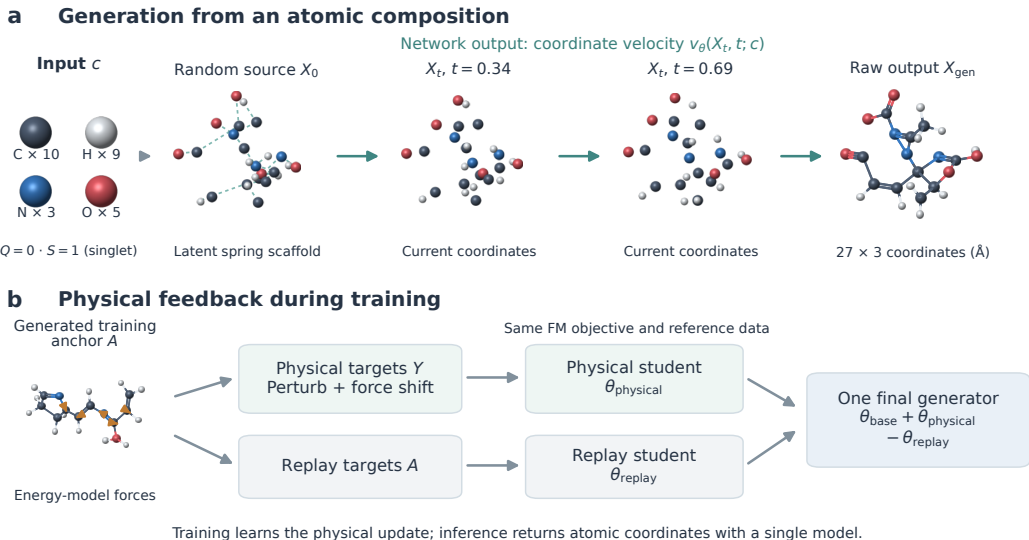
Figure 1: LatentSpring’s inputs, outputs and physical learning. (a) An actual recorded flow for C_{10}H_9N_3O_5 . The source supplies random coordinates X_0 ; the network reads current coordinates, flow time and composition, and predicts movement vectors. Solid bonds are inferred only for the displayed final output; dashed source edges are auxiliary springs. (b) A generated training anchor from a separate composition supplies local physical targets and matched replay targets. Their learned parameter difference updates one generator. All displayed molecular coordinates are unoptimized.
