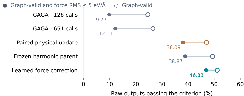
Figure 11: Graph support and physical quality on the same compositions. Open circles count graph-valid outputs; filled circles also require GFN2 force RMS at most 5 eV/Å. The gap shows graph-valid outputs above that force threshold. Every denominator includes all 512 attempts. The models have the distinct training histories and inference costs described in the text.
