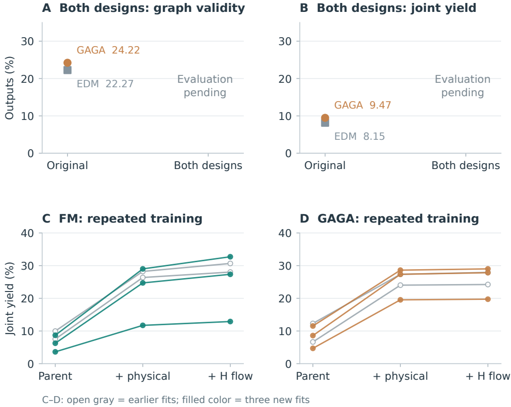
Figure 4: Transfer and training replication. (A–B) Original diffusion baselines and the combined-design comparison on 64 compositions, with two fits and 2,048 outputs per setting. Combined-design evaluation is pending; no outcome markers or connecting lines are drawn for it. The GAGA baseline here uses the two paired fits, while Figure 2 averages five. (C–D) Every fit from the completed physical-correction and hydrogen-readout study. Gray open markers identify the two earlier fits; colored filled markers identify the three new fits. Each line follows the same parent. These lower panels use the head fitted to each parent and do not include the combined-design diffusion experiment.
