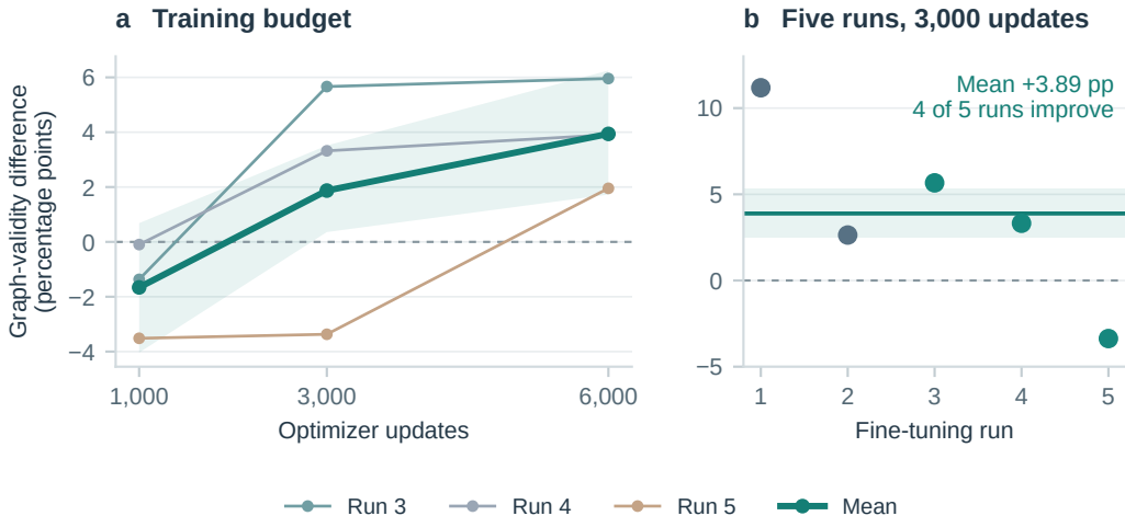
Figure 6: Source effects across training budgets and fine-tuning runs. Thin lines show all three new runs; the thick line is their mean. The right panel includes all five runs at 3,000 updates. Shading and the horizontal bar show 95% composition-bootstrap intervals conditional on the fitted models.
