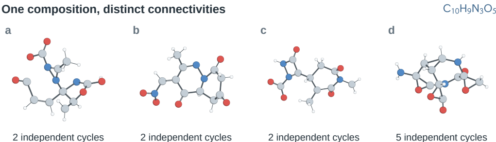
Figure 7: Different connectivities generated from the same atomic composition by the paired-update variant of LatentSpring. The initial trees have no cycles, but the generated molecules can contain rings. We show the first four graph-valid outputs with distinct connectivities for the first CHON composition with valid outputs in run 1 of the 24-composition set. Examples are not selected by energy or altered by geometry optimization. The number of independent cycles is the inferred edge count minus the atom count plus one.
