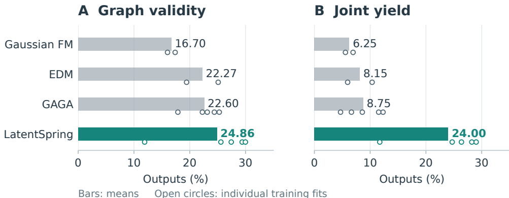
Figure 2: Complete generators on 64 unseen compositions. Bars give mean graph validity (A) and joint yield (B); open circles show every training fit. Gaussian FM and EDM use two fits (2,048 outputs each); GAGA and LatentSpring use five (5,120 each). All attempts are counted. LatentSpring uses the source and physical correction, without the optional hydrogen readout.
