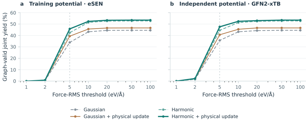
Figure 7: Joint graph-validity and residual-force yield for both sources, with and without the paired physical update. The denominator includes every raw generation attempt. Each threshold is applied to the RMS atomic-force magnitude in \text{eV}/\text{\AA} , and both potentials use the same threshold grid. No coordinates are optimized before evaluation.
