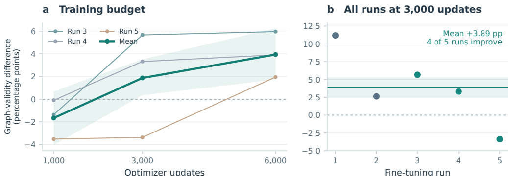
Figure 4: Source effects across training budgets and fine-tuning runs. Thin lines show all three new runs; the thick line is their mean. The right panel includes all five runs at 3,000 updates. Shading and the horizontal bar show 95% composition-bootstrap intervals conditional on the fitted models.
