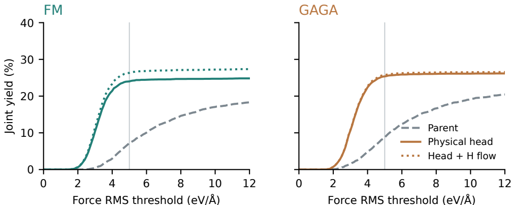
Figure 9: Joint yield as the force threshold varies, averaged over all five fits. The vertical reference marks the prespecified 5 eV/Å endpoint. These curves are descriptive; no threshold is selected from them.
