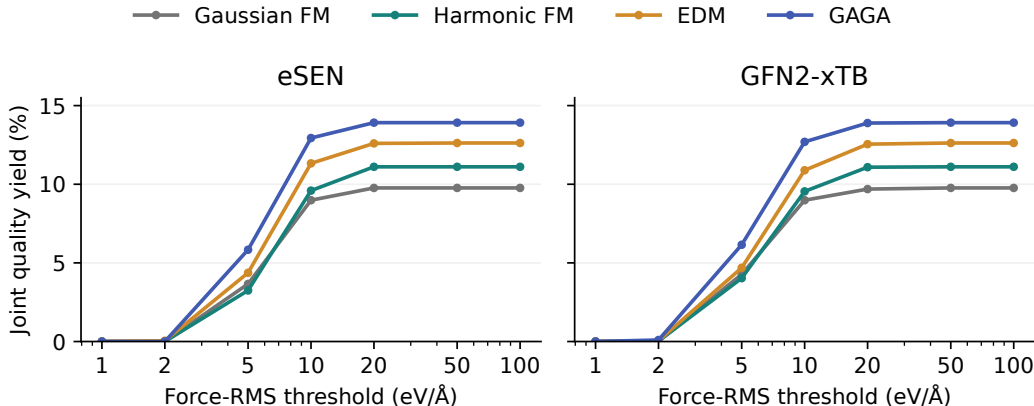
Figure 13: Fraction of all attempts that are graph-valid and have force RMS below the indicated threshold. Curves pool both independent initializations and all 64 compositions. GAGA has the highest pooled yield at most nontrivial thresholds under both potentials.
