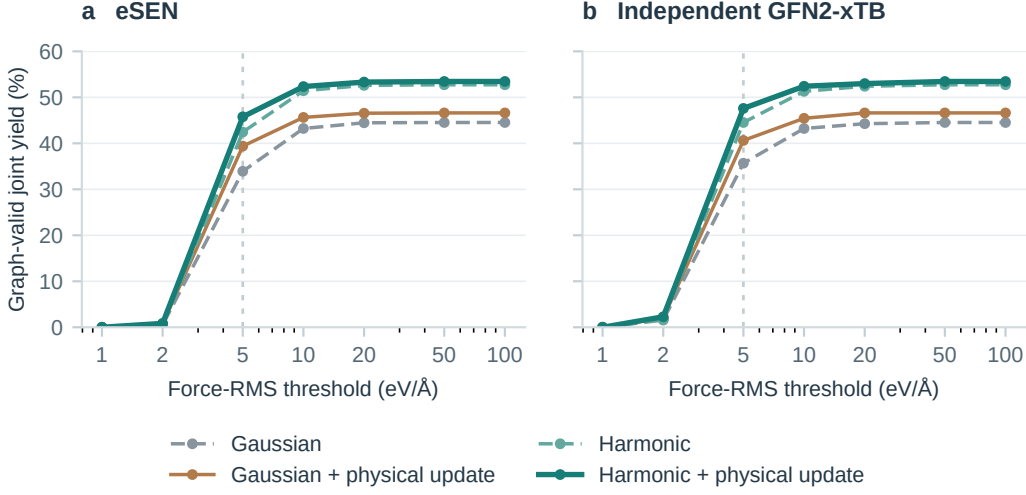
Figure 14: Joint graph-validity and residual-force yield for both sources, with and without the paired physical update. The denominator includes every raw generation attempt. Each threshold is applied to the RMS atomic-force magnitude in \text{eV}/\text{\AA} , and both potentials use the same threshold grid. No coordinates are optimized before evaluation.
