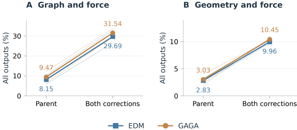
Figure 4: Transfer of both correction networks. Bold lines show the two-fit means; faint lines show each paired fit. Each setting uses 2,048 attempts on 64 compositions. The target retains its original source and backbone, and the hydrogen readout is disabled. (A) Graph-and-force yield. (B) The stricter geometry-and-force yield.
