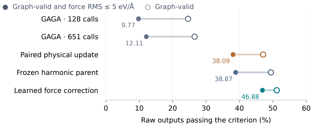
Figure 11: Graph support and physical quality on the same compositions. Open circles count graph-valid outputs; filled circles also require GFN2 force RMS at most 5 eV/Å. The gap shows graph-valid outputs above that force threshold. Every denominator includes all 512 attempts. The models have the distinct training histories and inference costs described in the text.
