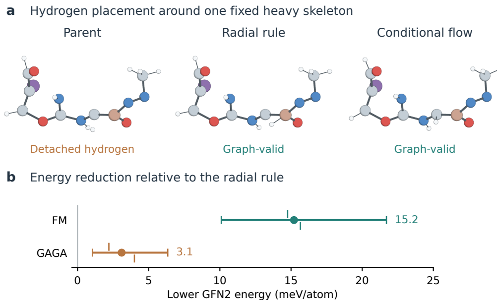
Figure 10: A conditional hydrogen flow learns more than attachment distance. Top: the same saved FM output before readout, after the radial rule, and after the learned flow. All atoms are shown with a shared camera and scale. Sticks are distance contacts in every panel, not inferred chemical bond orders. The example is selected by a fixed metadata hash among repaired, jointly graph-valid examples with at most 28 atoms; energy is not a selection criterion. Bottom: all-output energy reductions relative to the radial rule, with 95% composition-bootstrap intervals and the two fit-specific means. Carbon, hydrogen, nitrogen, oxygen, boron, and iodine are gray, white, blue, red, tan, and purple.
