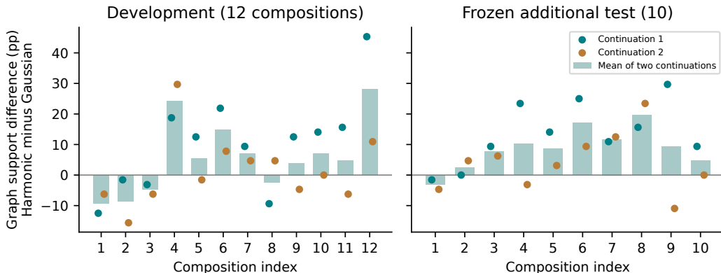
Figure 6: Harmonic-minus-Gaussian graph-validity differences for each composition. Points show the two individual fine-tuning runs, and bars show their mean. Gains vary across compositions and runs. Both evaluation sets use the same trained models.
