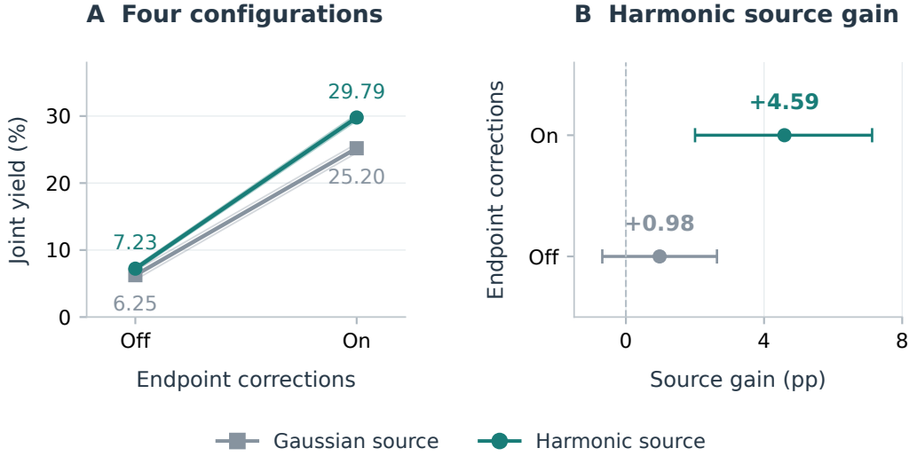
Figure 3: Contributions of the source and endpoint corrections. (A) Mean joint graph-and-force yield for four settings; faint lines retain both fits. (B) Harmonic-minus-Gaussian gains, with nominal 95% intervals from resampling fits and compositions. Each setting uses 2,048 outputs on the same 64 compositions.
