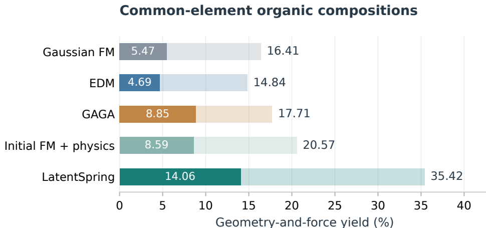
Figure 5: Raw generation on 12 common-element organic compositions. Each full bar shows geometry-and-force yield; the darker portion additionally requires zero assigned atom charges. All 384 attempts per method remain in the denominator.
