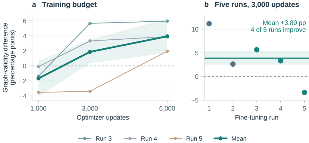
Figure 7: Source effects across training budgets and fine-tuning runs. Thin lines show all three new runs; the thick line is their mean. The right panel includes all five runs at 3,000 updates. Shading and the horizontal bar show 95% composition-bootstrap intervals conditional on the fitted models.
