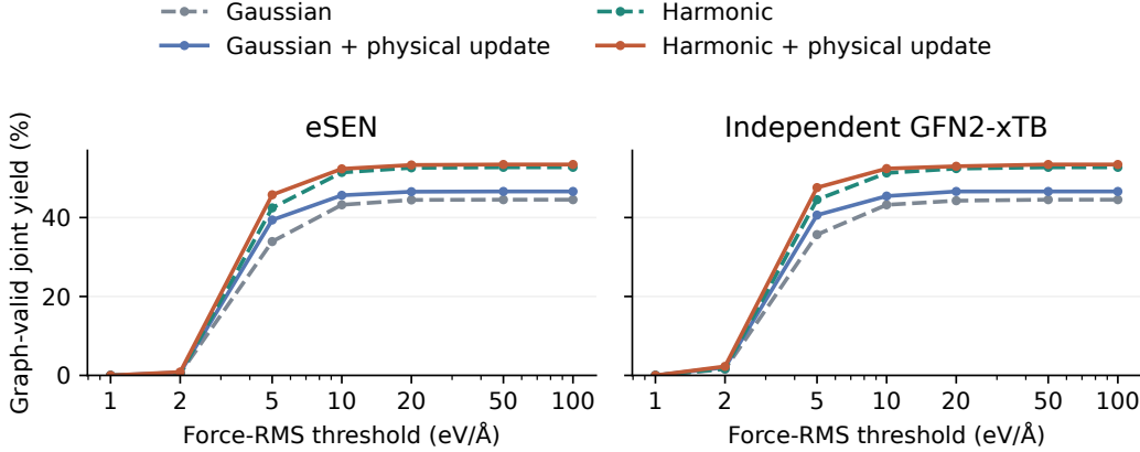
Figure 6: Joint chemical-graph and residual-force yield for each source and physical-update setting. Every attempted raw output contributes to the denominator. The threshold is applied to the RMS atomic-force magnitude in eV/Å; no geometry optimization precedes either readout. Points use the same threshold grid under both potentials.
