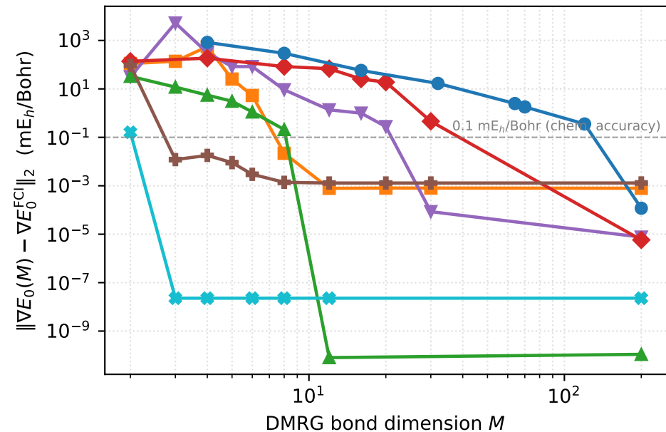
(a) Analytic gradient error
