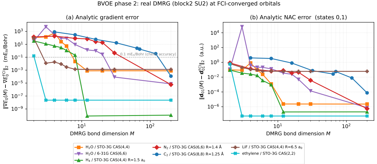
Figure 2: Fixed-orbital bond-dimension response-error convergence for public benchmark systems. Gradient errors are reported in mE_h/\text{Bohr} and nonadiabatic coupling errors in atomic units.
