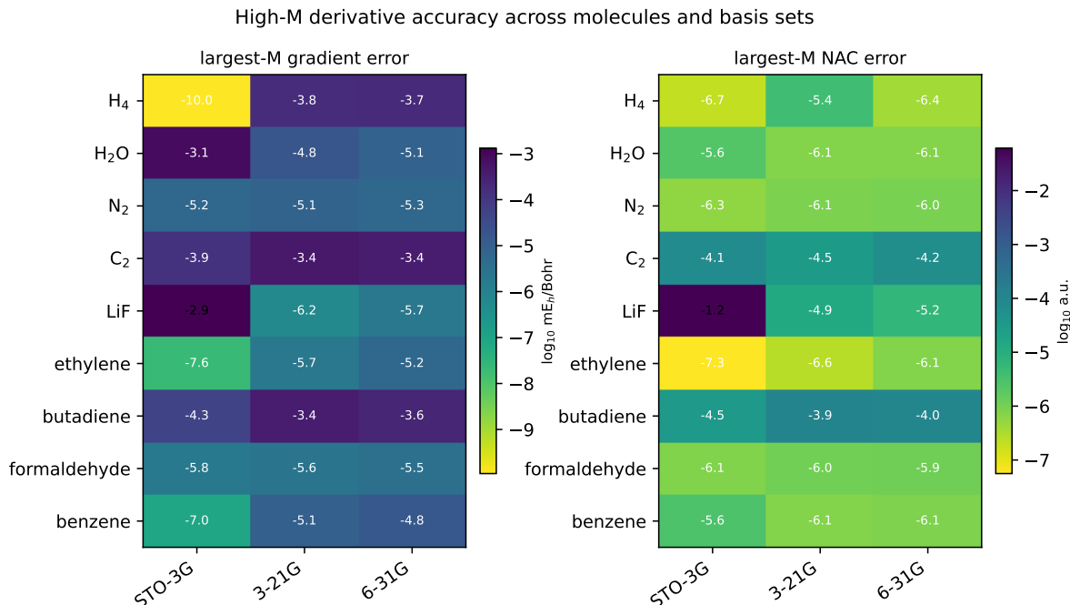
Figure 3: Largest- M derivative errors across the public molecule/basis matrix. Each entry is the base-10 logarithm of the largest- M gradient error in mE_h/\text{Bohr} or NAC error in atomic units.
