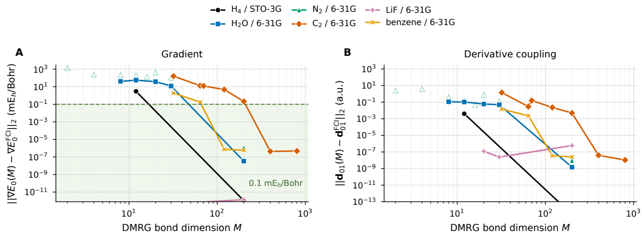
Figure 3: Fixed-orbital bond-dimension response-error convergence for public benchmark systems. Gradient errors are reported in mE h /Bohr and nonadiabatic coupling errors in atomic units. Filled symbols connected by lines pass the uniform benchmark QC: minimum assigned root overlap with the FCI reference of at least 0.98 and converged gradient and NAC response equations. Pale open triangles mark computed N 2 /6-31G points that fail one of these QC filters and are not used for convergence claims.
