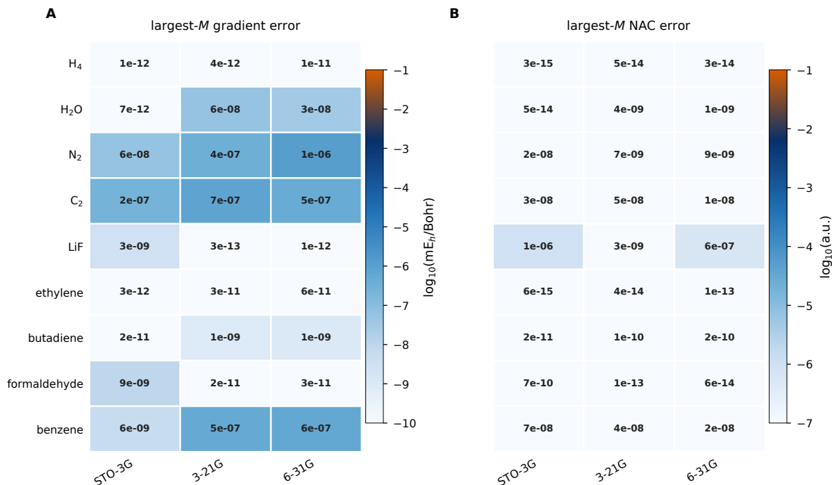
Figure 4: Largest- M derivative errors across the public molecule/basis matrix. Color encodes the base-10 logarithm of the error, while each cell reports the corresponding gradient error in \text{mE}_h/\text{Bohr} or NAC error in atomic units.
