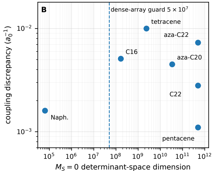
MPS-overlap coupling finite differences
