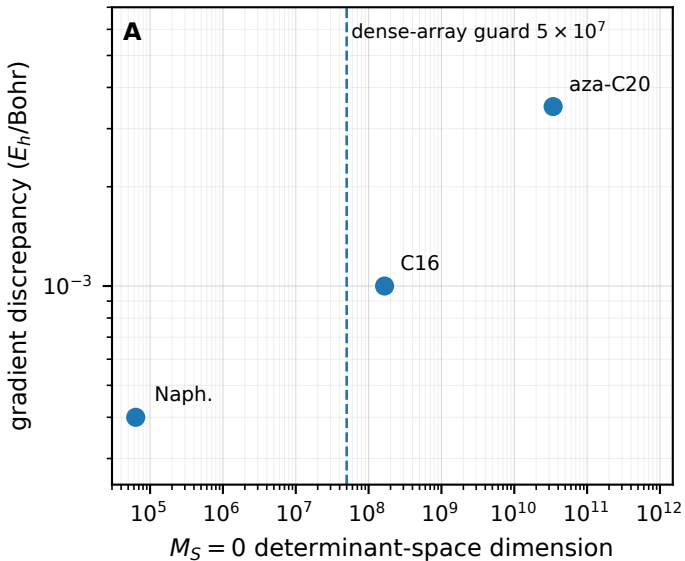
Gradient finite differences
