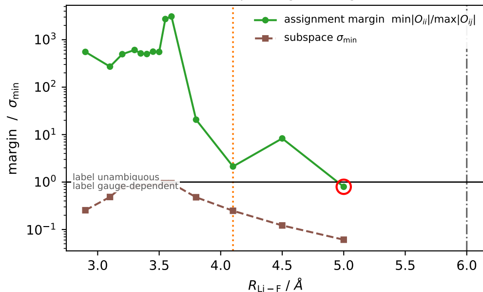
(d) where a root LABEL stops being meaningful
