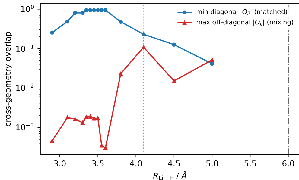
(c) matched vs mixing overlap
