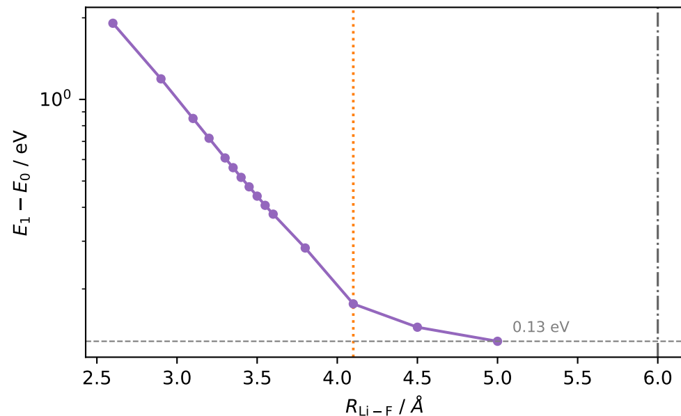
(b) gap closes 1.91 \rightarrow 0.13 eV
