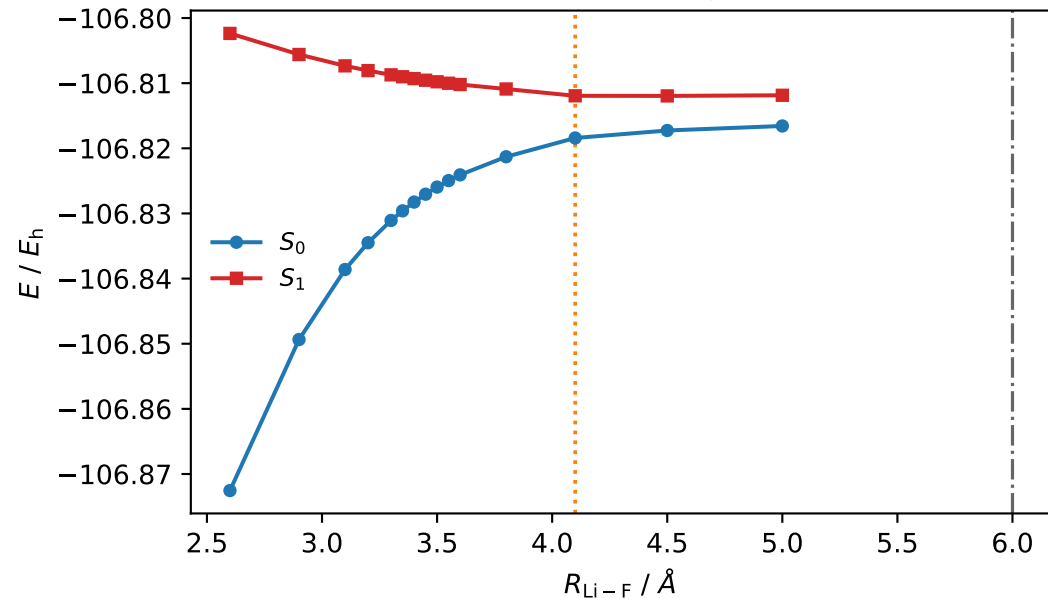
(a) SA(2)-CASSCF(6,6) avoided crossing
