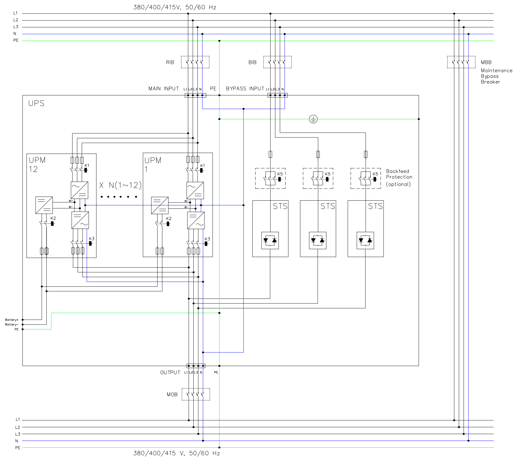
9395XR-1500 UPS Wiring Diagram
