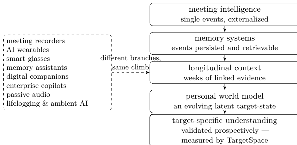
Figure 1: The convergence ladder. Today’s product categories (left) start from different capture problems but climb the same ladder (right): externalized events become persistent memory, memory becomes longitudinal context, context becomes a personal world model, and the model’s claim to target-specific understanding is validated — or not — by prospective forecasting. TargetSpace is the shared measurement layer at the top rung; the placement of categories is illustrative, not a ranking.
