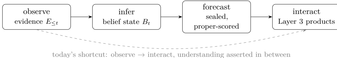
Figure 2: One sequence, two paths. The benchmark scores only the third step — the sealed forecast — because it is the step where a claimed model of the person either survives contact with the future or does not.
