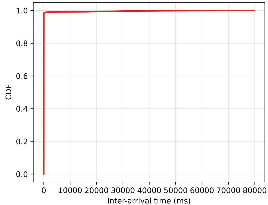
3GPP HTTP downlink inter-arrival CDF
