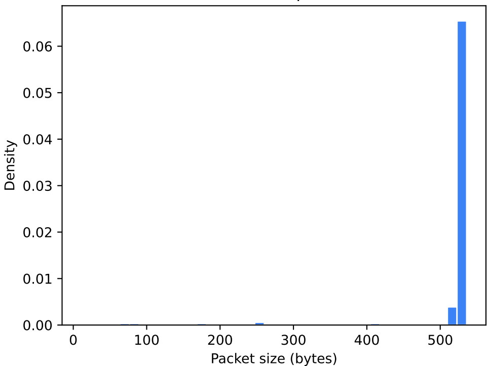
3GPP HTTP downlink packet size PDF
