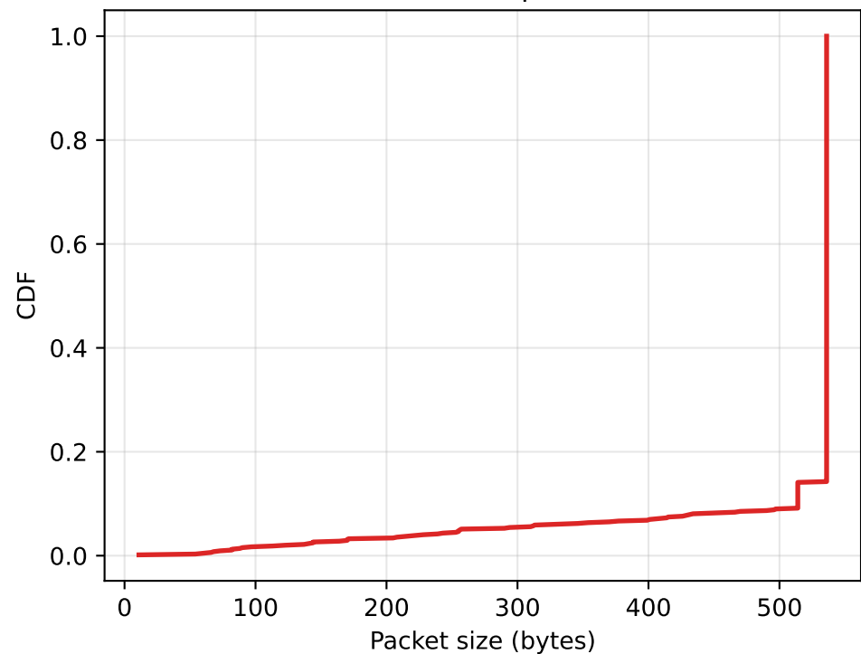
3GPP HTTP downlink packet size CDF
