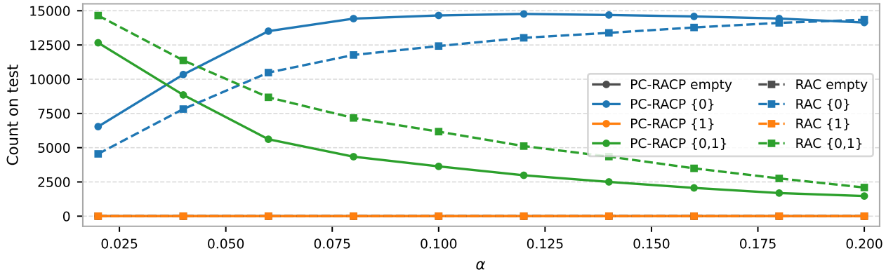
Prediction-set counts given action a=0
