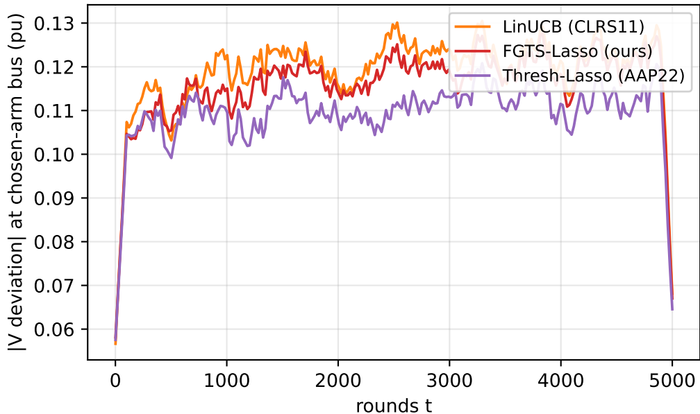
Voltage-deviation magnitude (top 3 algos)
