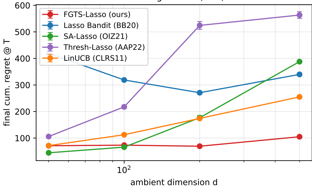
Final regret vs d ( s=5 )
