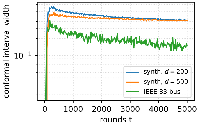
(b) Interval width vs t
