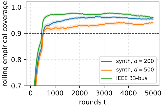
(a) Coverage at level 1 - \alpha = 0.9
