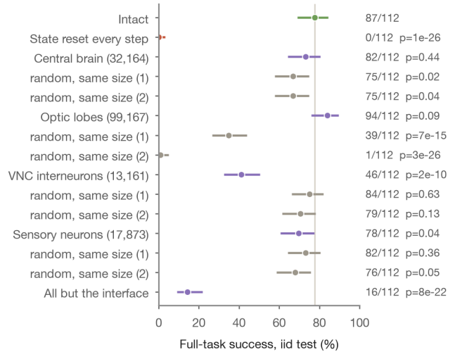
Figure 4: Test-time lesions of the reported controller: full-task success on 112 iid test episodes with Wilson 95% intervals, and exact McNemar p against intact on the same episodes. Purple: an anatomical group silenced (neuron count); grey: random non-interface sets of the same size.
