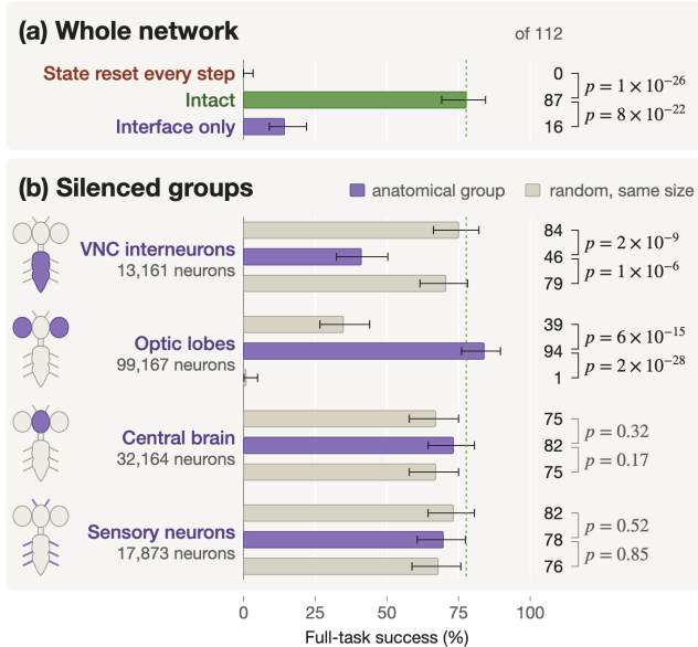
Figure 4: Test-time lesions of the reported controller on 112 iid test episodes: full-task success with Wilson 95% intervals and the number of successful episodes; the dashed line is intact. (a) The recurrent state cleared before every control step, and only the interface neurons left. (b) Each anatomical group silenced (purple; schematic of the fly CNS with the group filled) between two random non-interface sets of the same size (grey). Brackets: exact McNemar p on the same episodes, against intact in (a) and of the anatomical lesion against each random set in (b).
