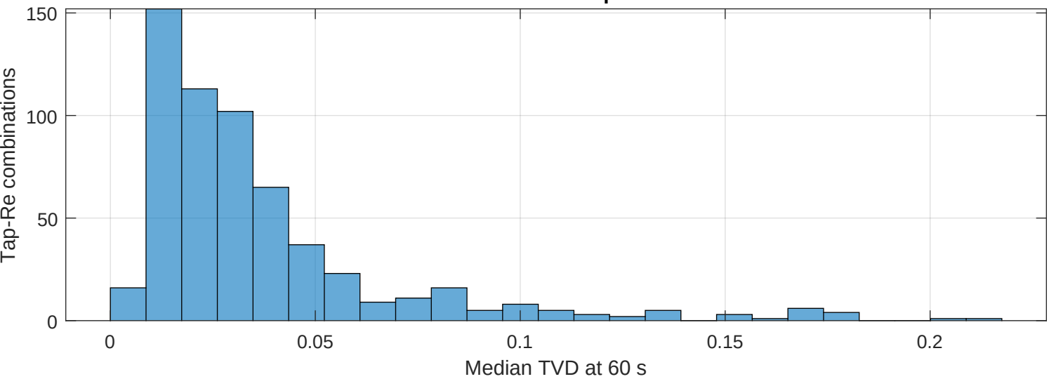
Distribution across all 588 tap-Re combinations
