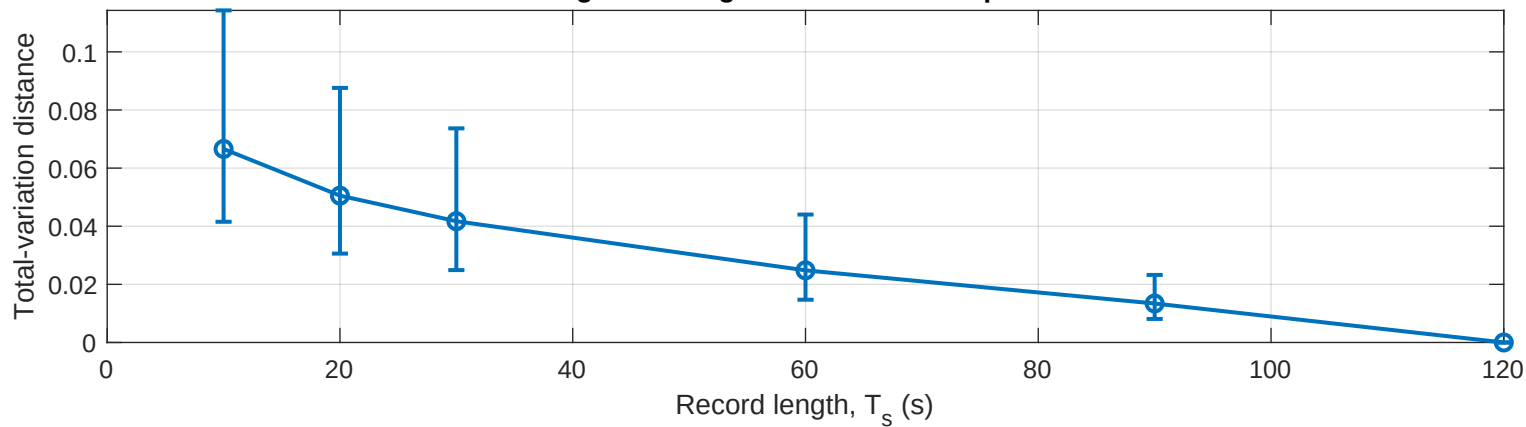
PDF record-length convergence across 588 tap-Re combinations
