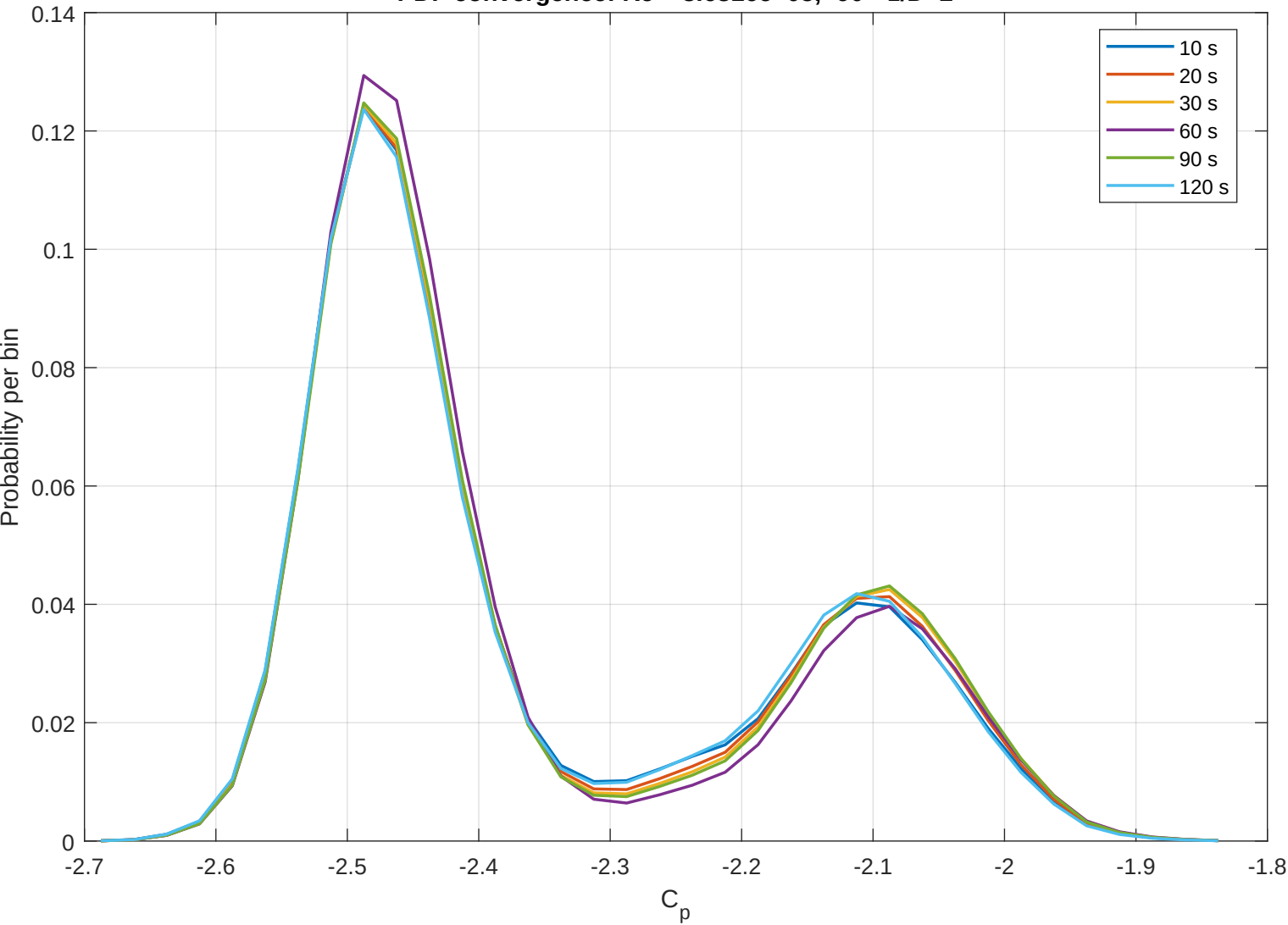
PDF convergence: Re = 3.6816e+05, -90° z/D=2
