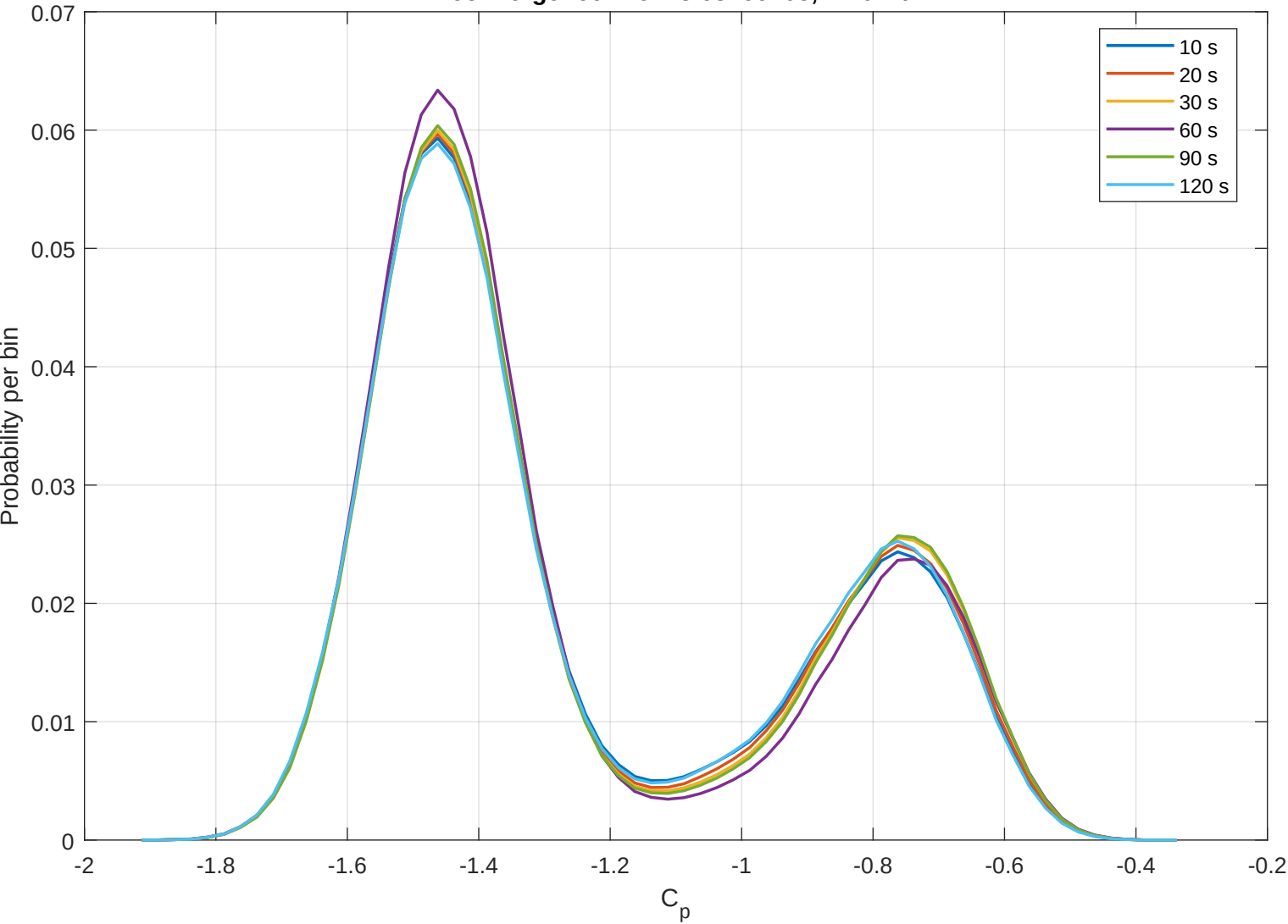
PDF convergence: Re = 3.6816e+05 , -110^\circ z/D=2
