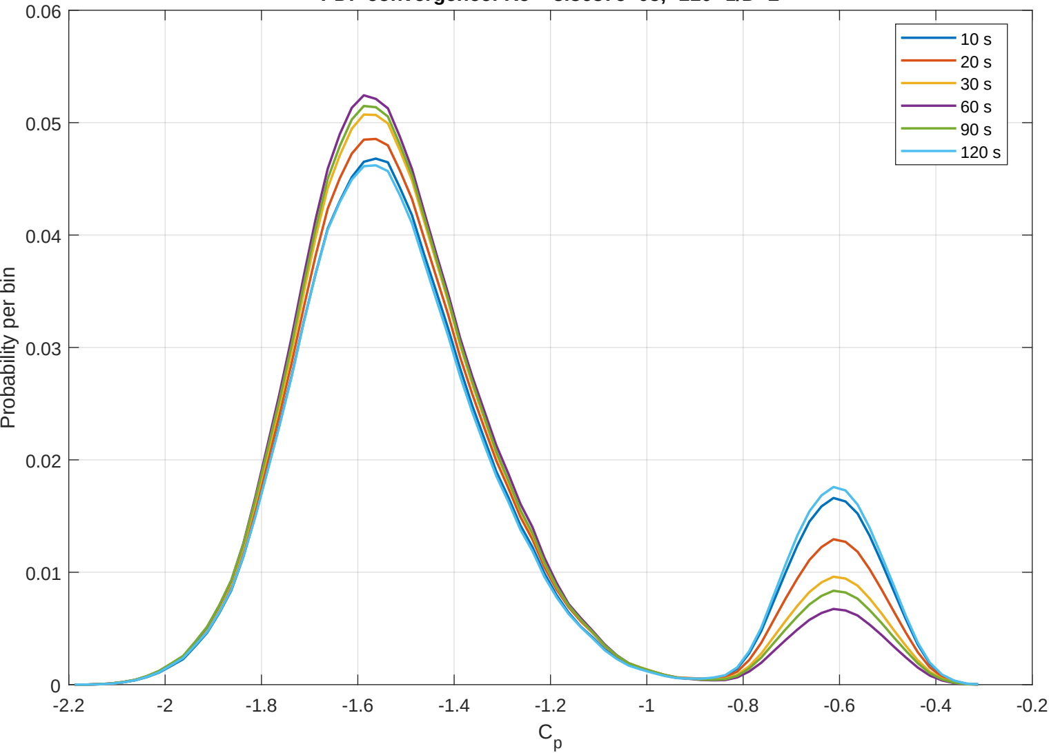
PDF convergence: Re = 3.3637e+05, -110° z/D=2
