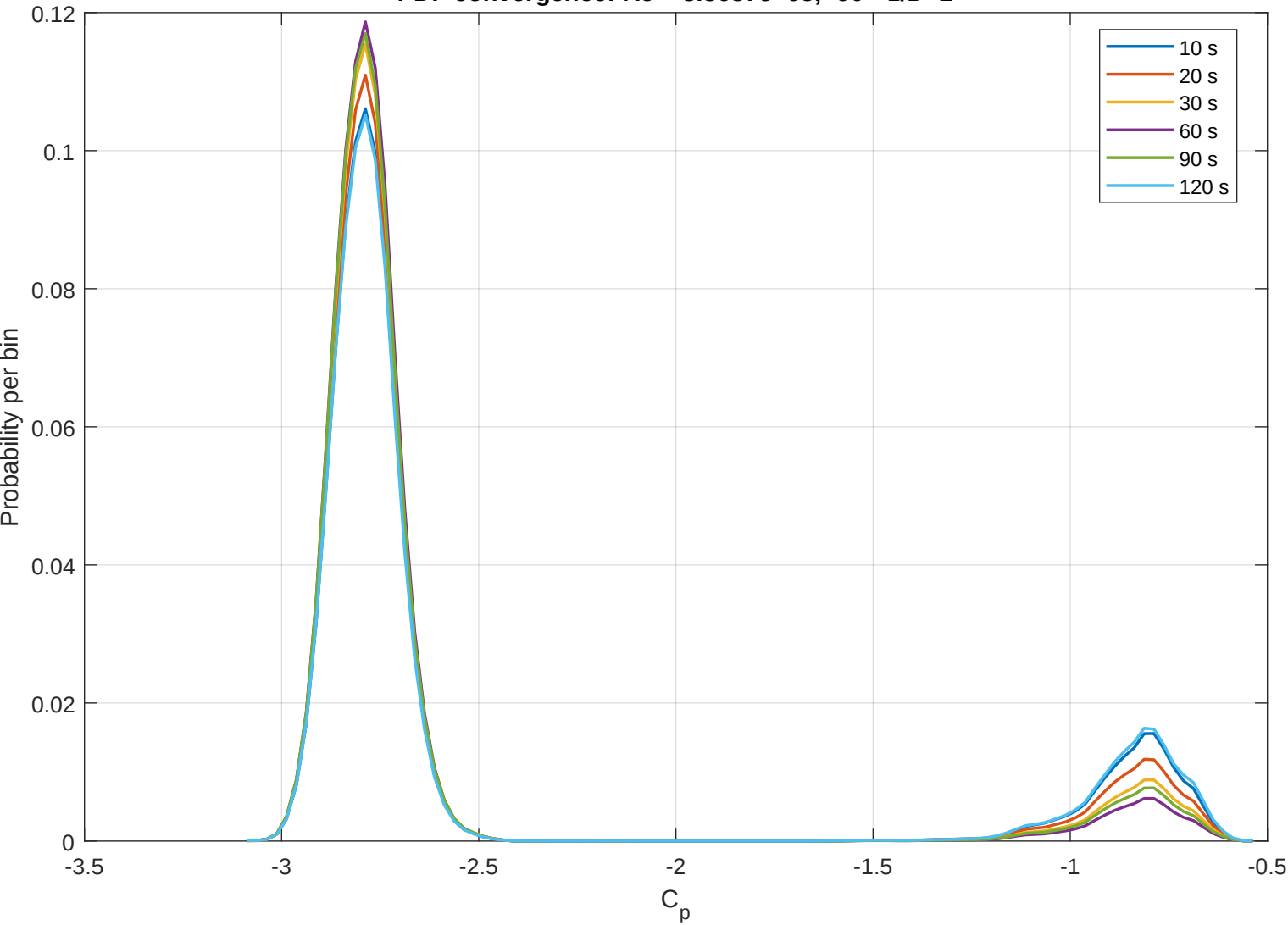
PDF convergence: Re = 3.3637e+05, -90° z/D=2
